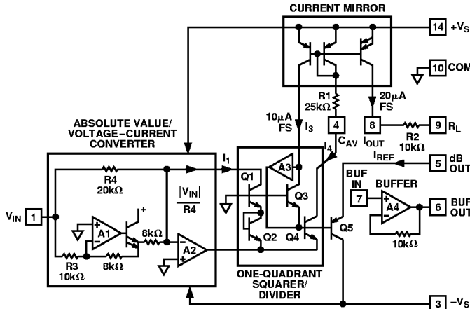
Figure 9. Simplified Schematic
