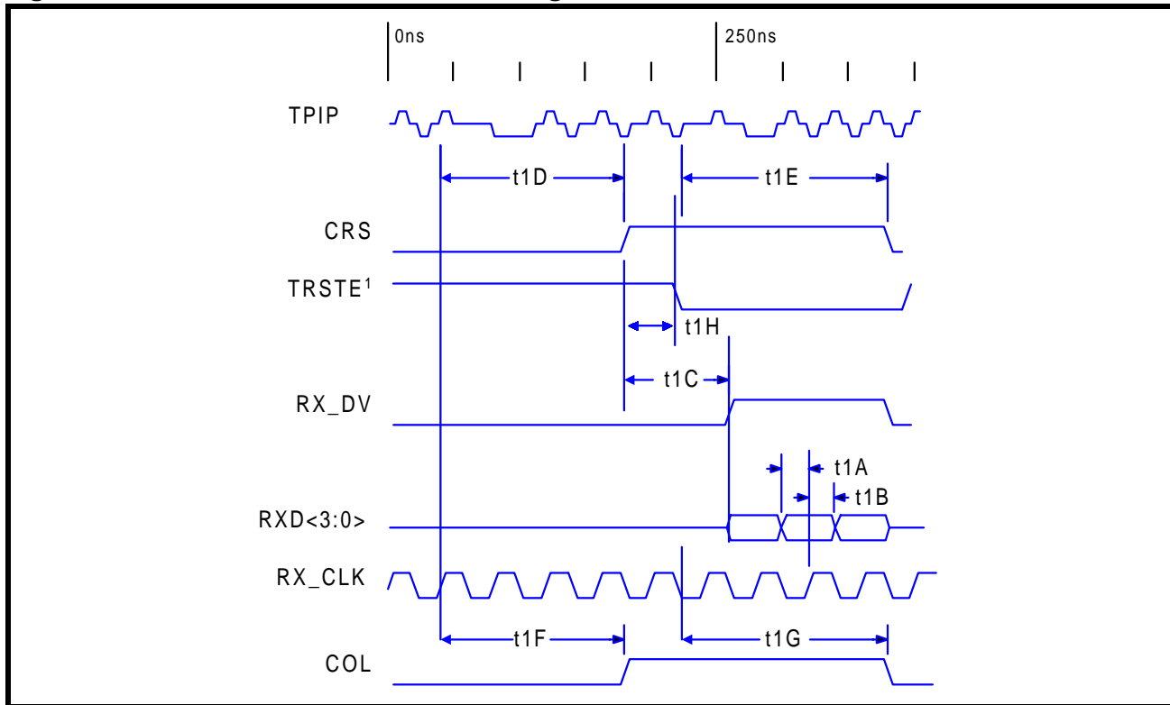
Figure 21: MII - 100BASE-TX Receive Timing / 4B Mode
