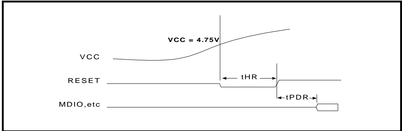
Figure 35: Power-Down Recovery Timing (Over Recommended Range)
