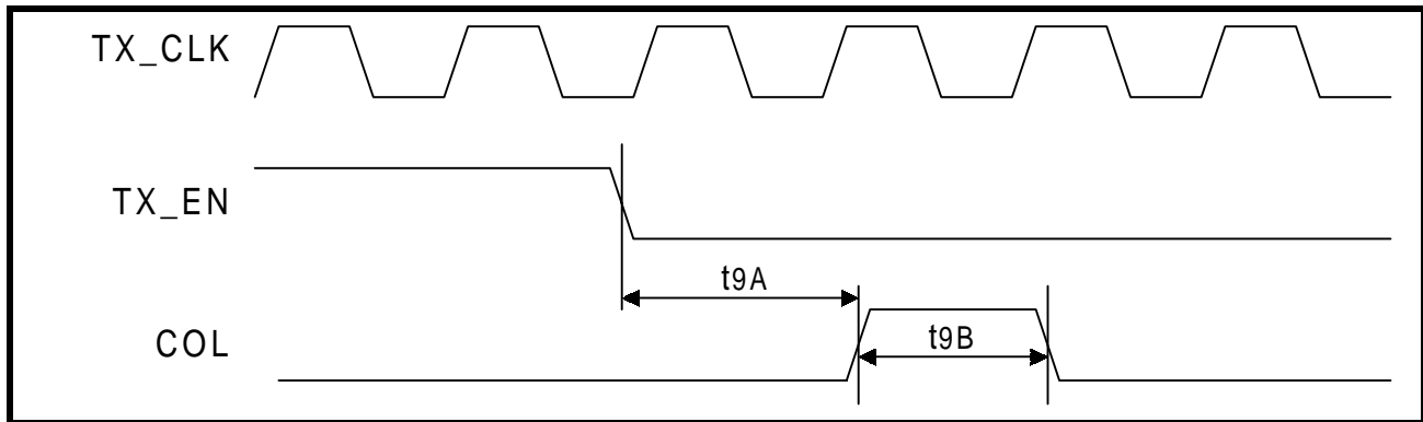
Figure 29: 10BASE-T SQE (Heartbeat) Timing
