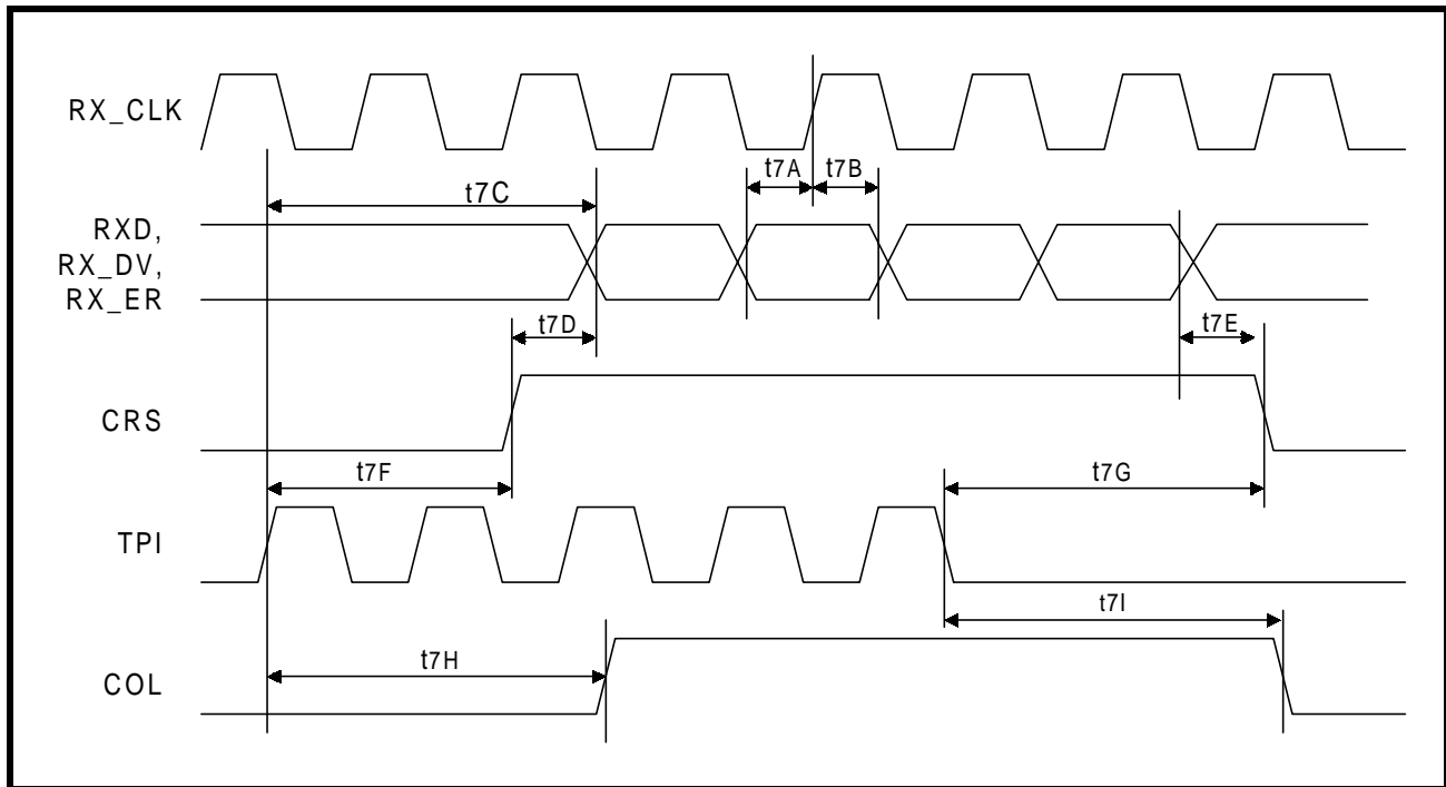
Figure 27: MII - 10BASE-T Receive Timing
