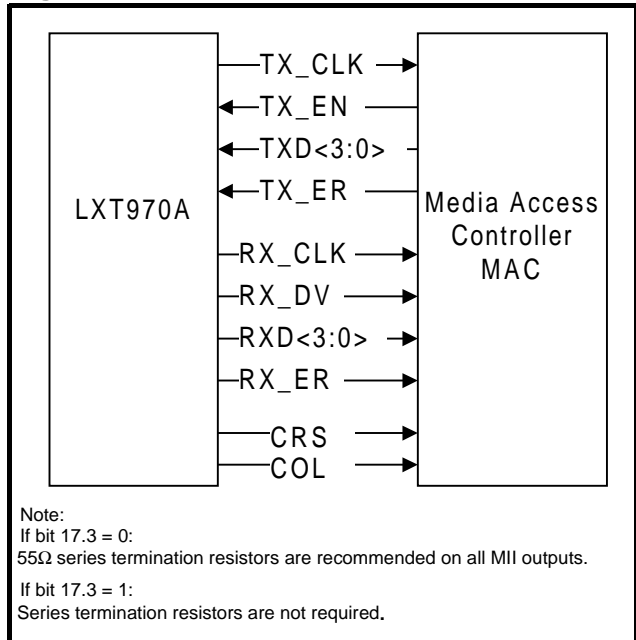
Figure 4: MII Data Interface
