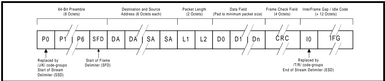
Figure 12: 100BASE-TX Frame Structure
