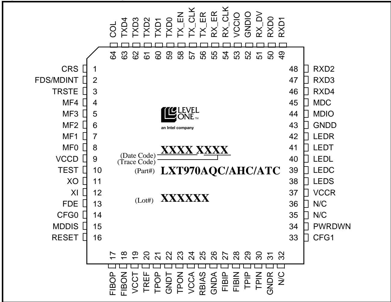
Figure 1: LXT970A Pin Assignments
