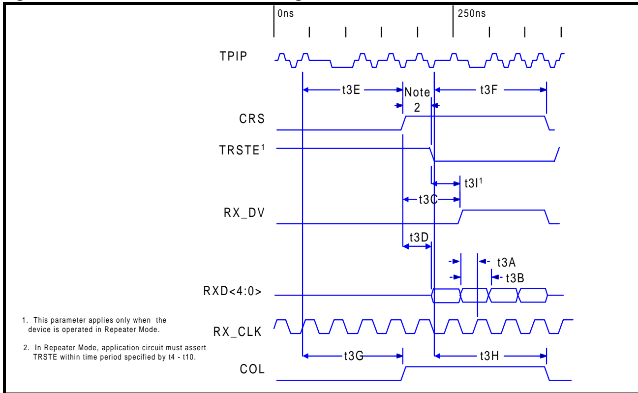
Figure 23: MII - 100BASE-TX Receive Timing / 5B Mode
