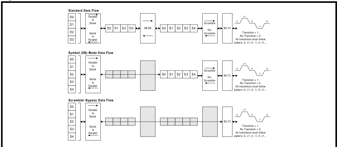
Figure 13: 100BASE-TX Data Flow
