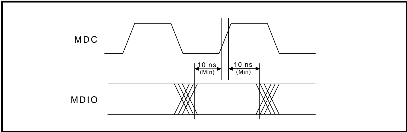
Figure 33: MDIO Timing when Sourced by STA
