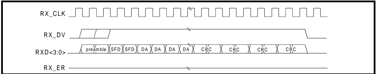
Figure 16: 100BASE-TX Reception with Invalid Symbol
