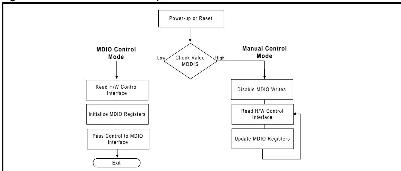
Figure 10: LXT970A Initialization Sequence
