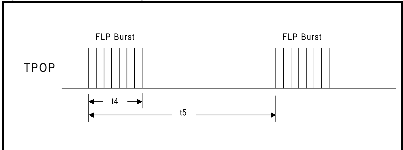
Figure 32: Fast Link Pulse Timing
