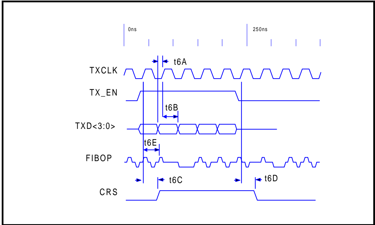
Figure 26: MII - 100BASE-FX Transmit Timing / 4B Mode
