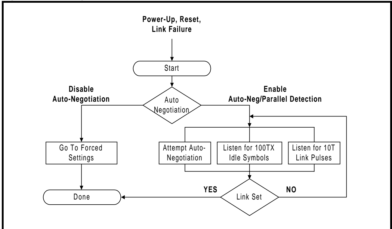
Figure 11: Auto-Negotiation Operation
