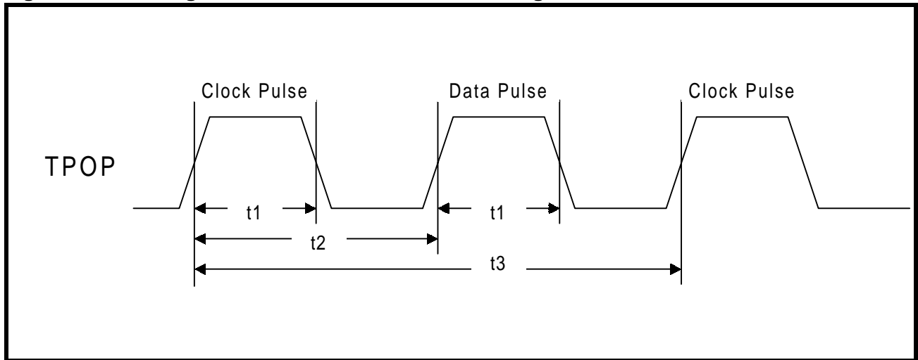
Figure 31: Auto Negotiation and Fast Link Pulse Timing
