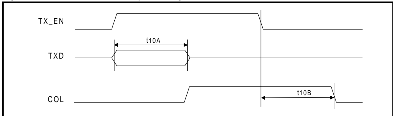
Figure 30: 10BASE-T Jab and Unjab Timing
