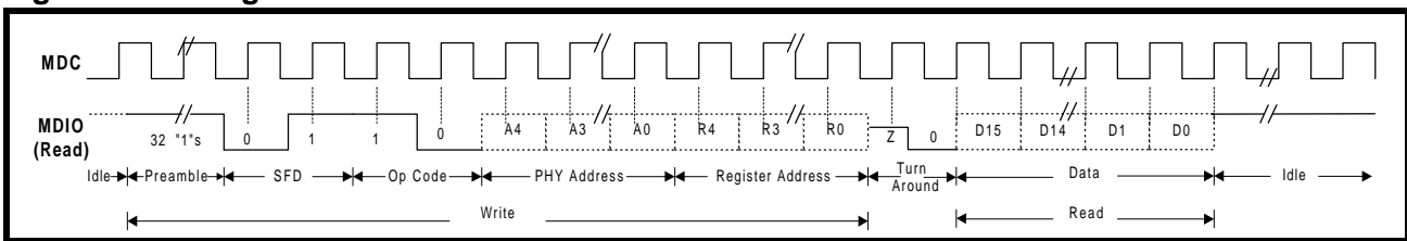
Figure 8: Management Interface - Read Frame Structure
