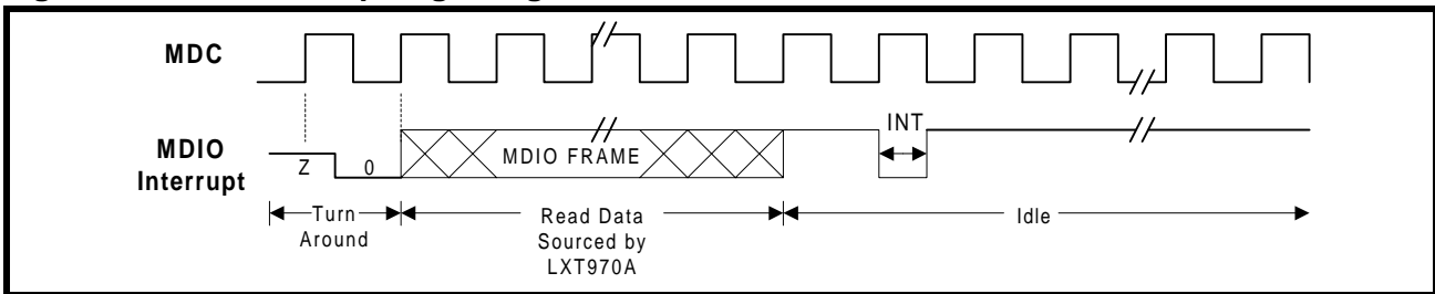
Figure 7: MDIO Interrupt Signaling
