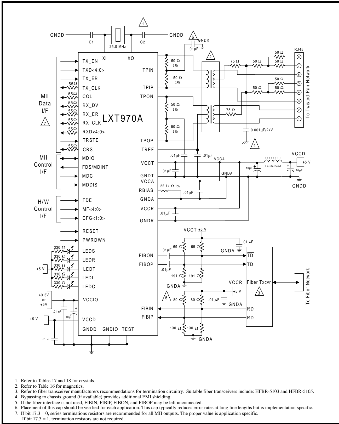
Figure 20: Typical Interface Circuitry
