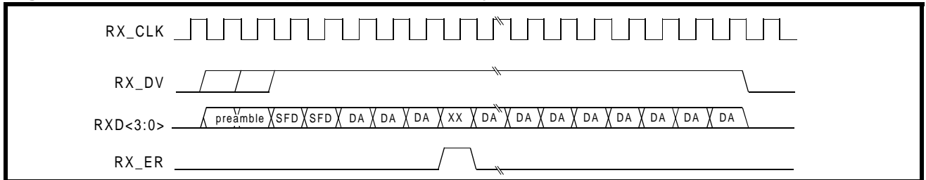
Figure 17: 100BASE-TX Transmission with No Errors
