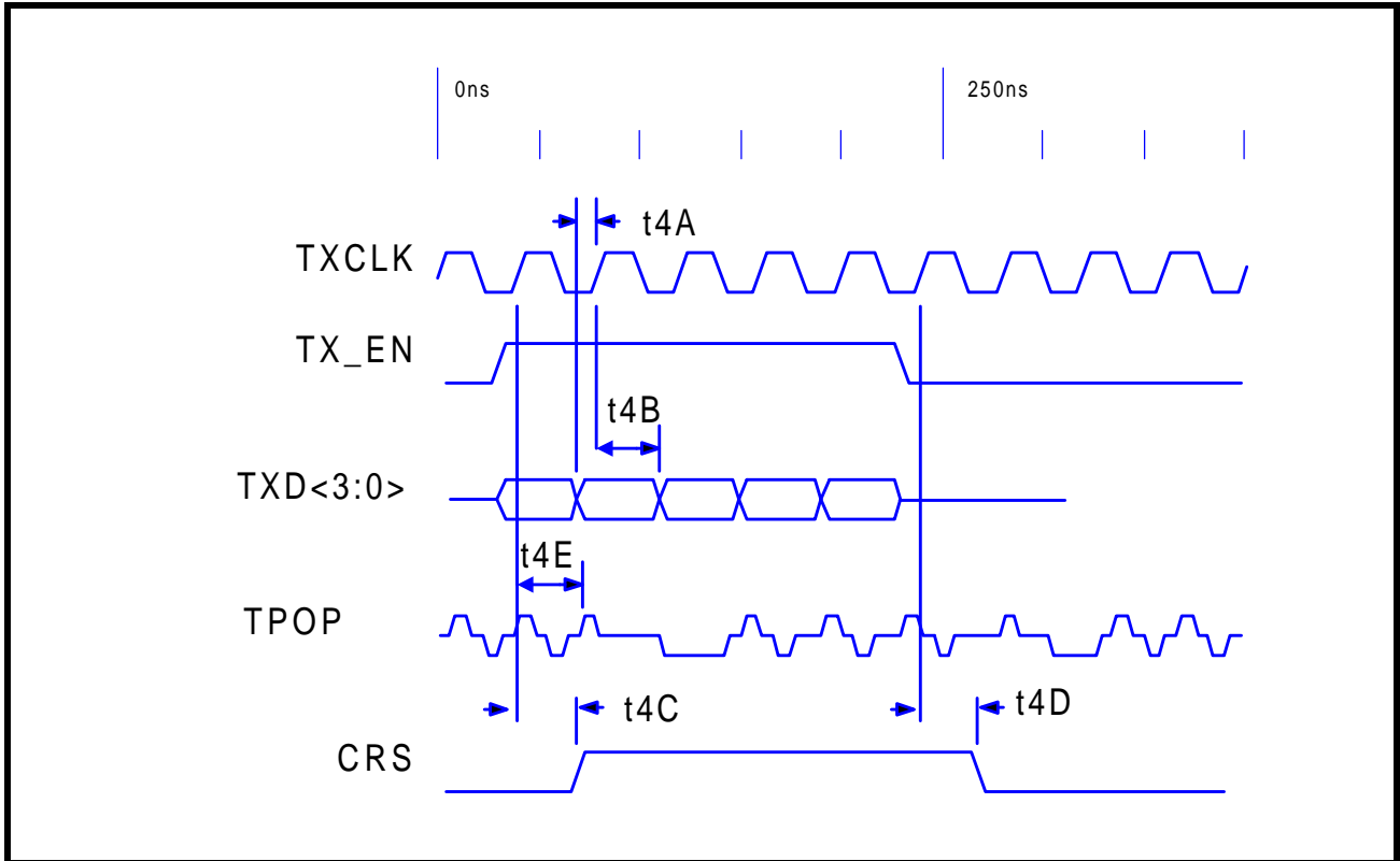
Figure 24: MII - 100BASE-TX Transmit Timing / 5B Mode
