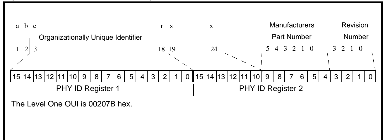
Figure 36: PHY Identifier Bit Mapping
