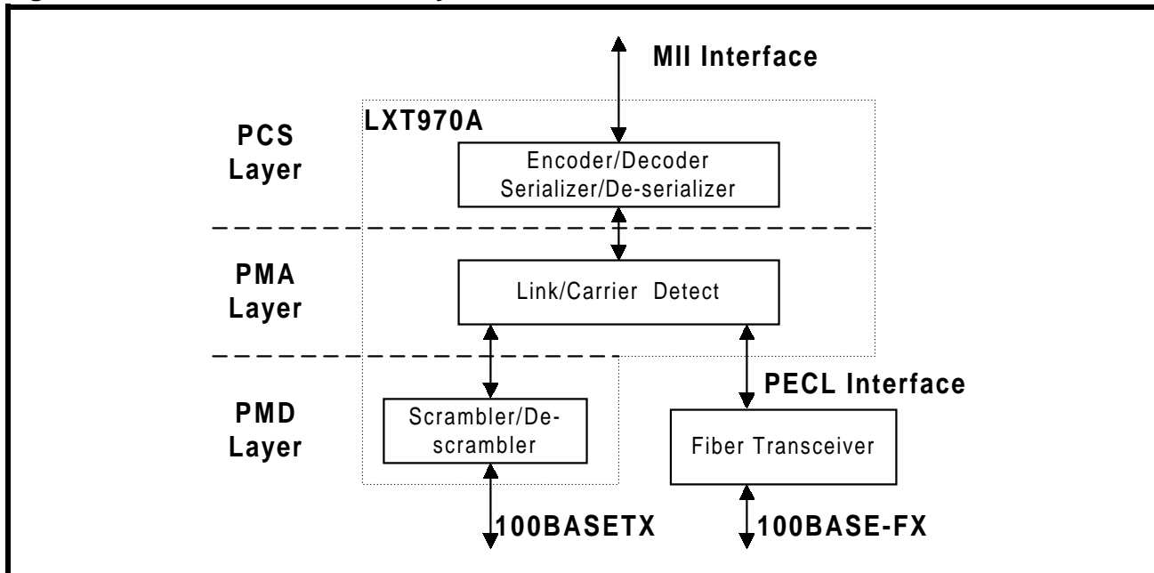
Figure 14: LXT970A Protocol Sublayers
