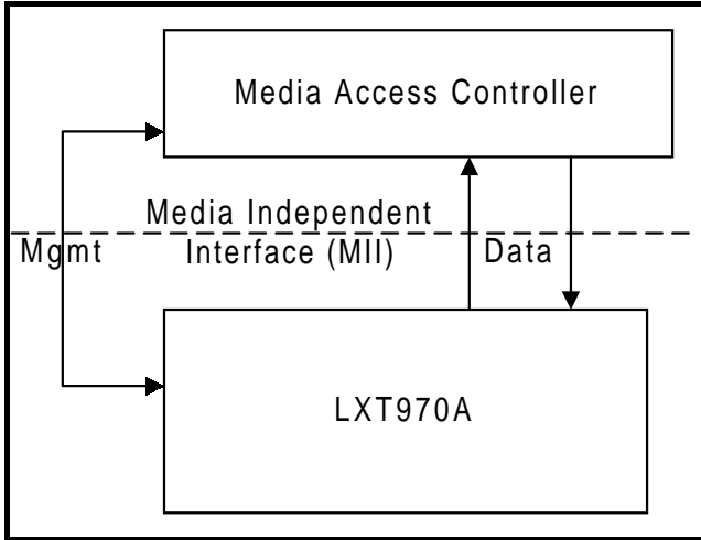
Figure 3: MII Interface
