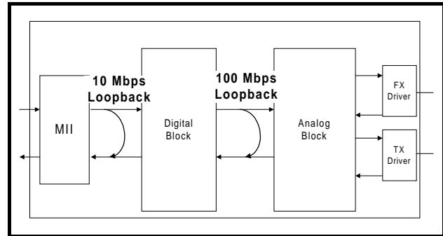
Figure 5: Loopback Paths
