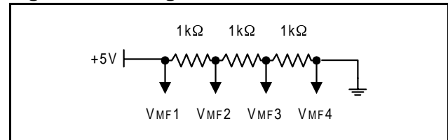
Figure 19: Voltage Divider
