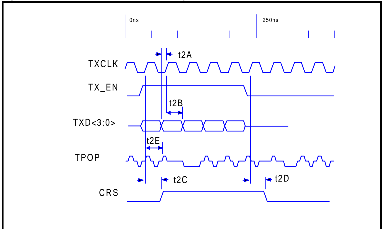
Figure 22: MII - 100BASE-TX Transmit Timing / 4B Mode
