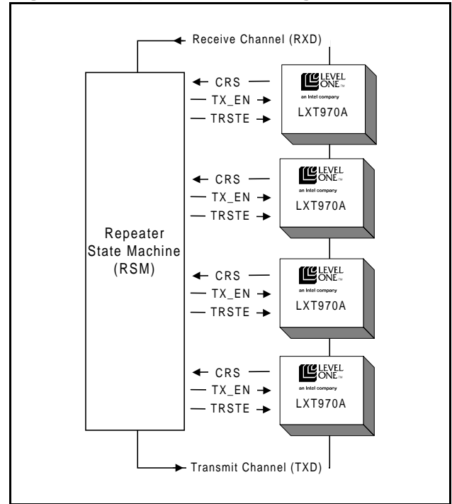
Figure 6: Repeater Block Diagram
