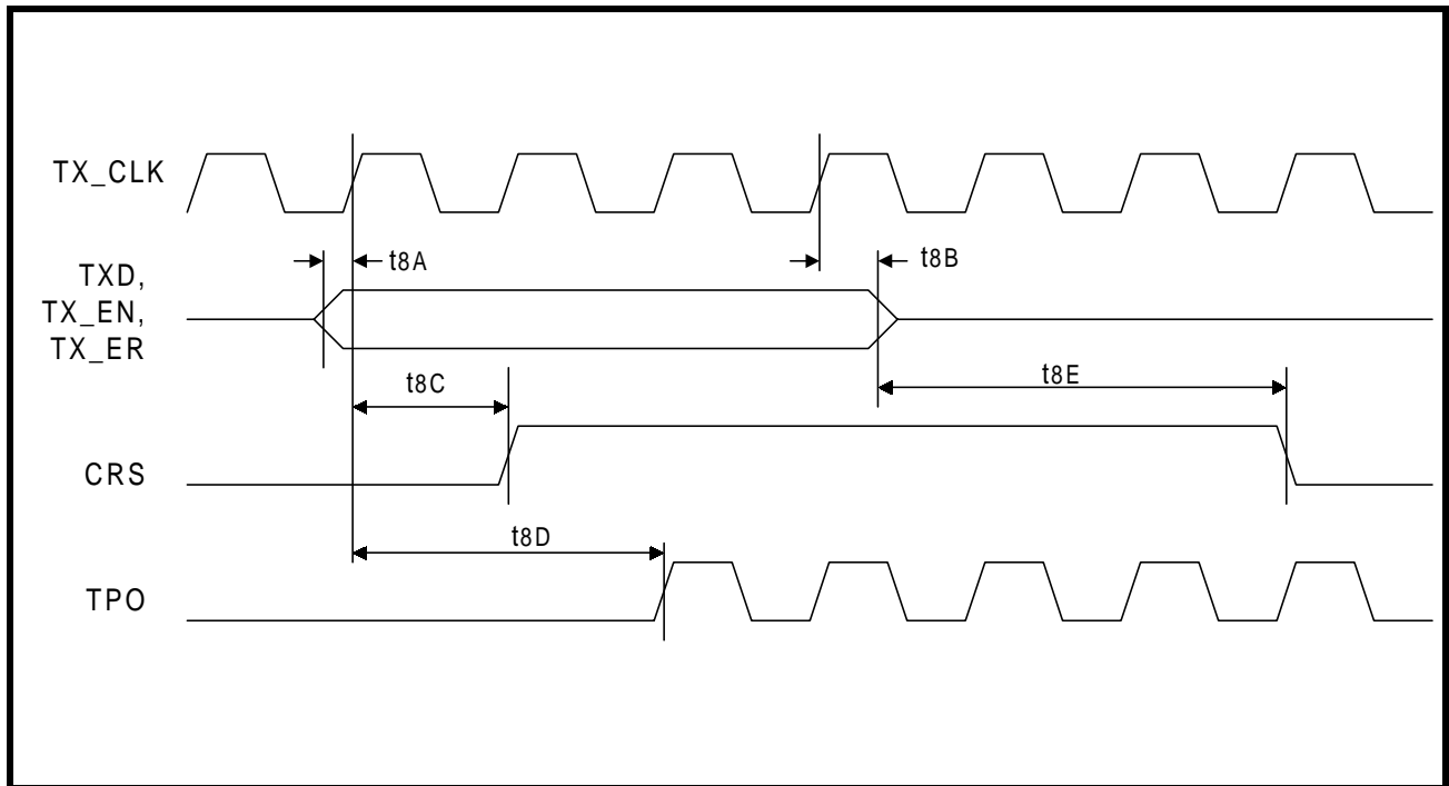
Figure 28: MII - 10BASE-T Transmit Timing
