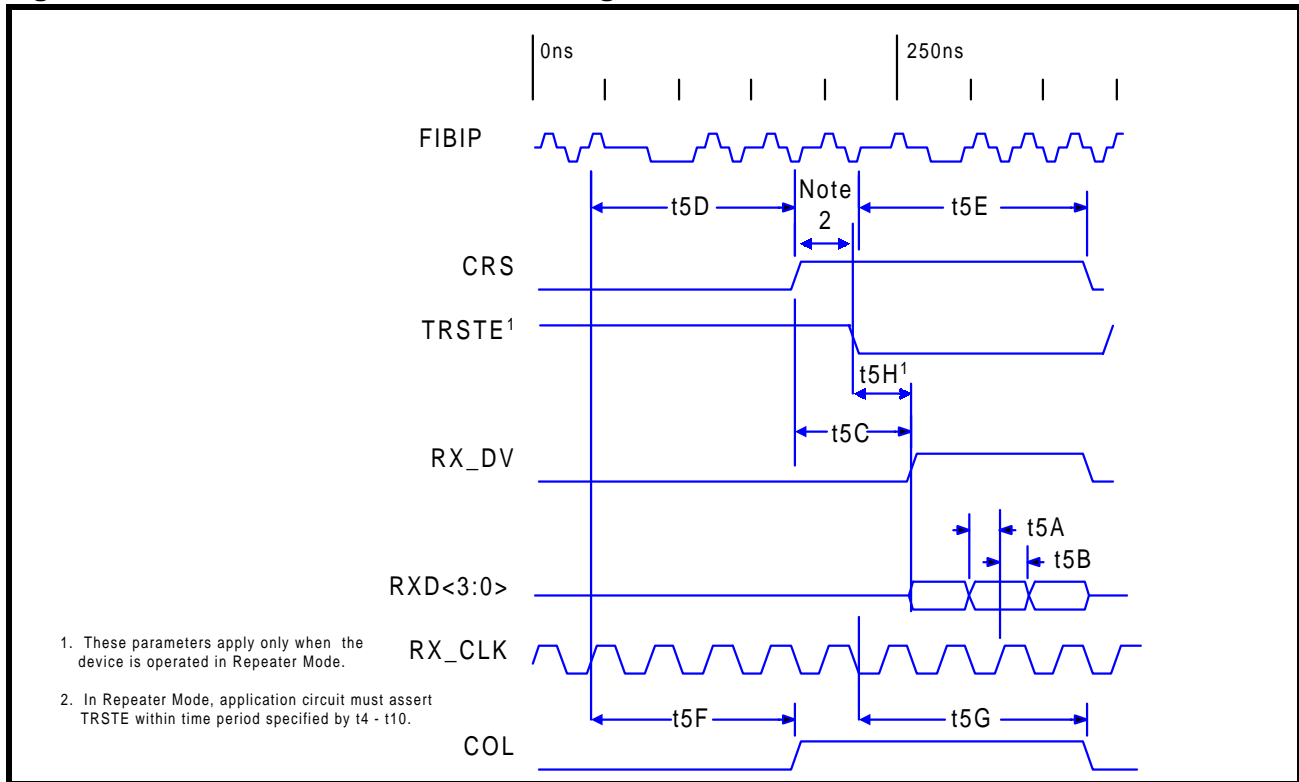
Figure 25: MII - 100BASE-FX Receive Timing / 4B Mode
