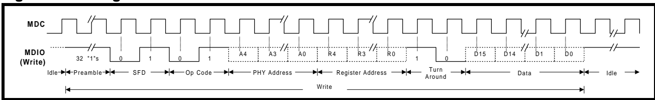
Figure 9: Management Interface - Write Frame Structure
