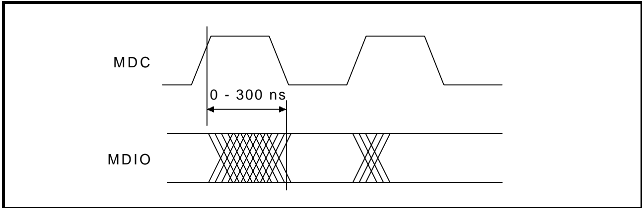
Figure 34: MDIO Timing when Sourced by PHY
