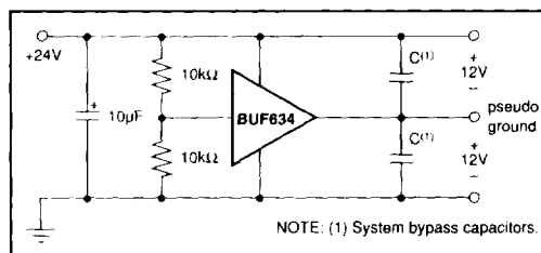
FIGURE 5. Pseudo-Ground Driver.
