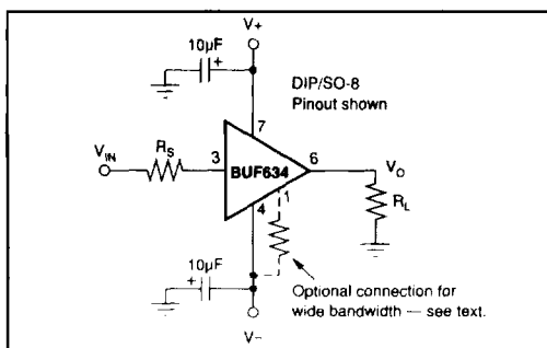
FIGURE 2. Buffer Connections.
