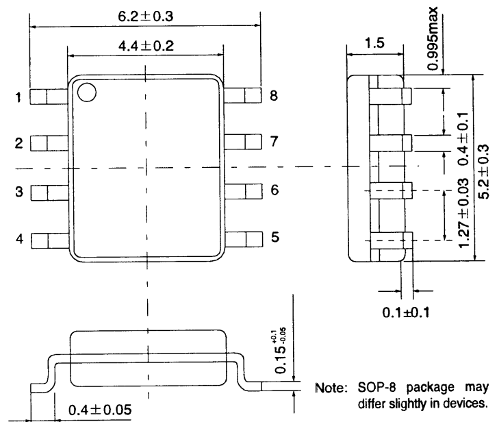
SOP-8
