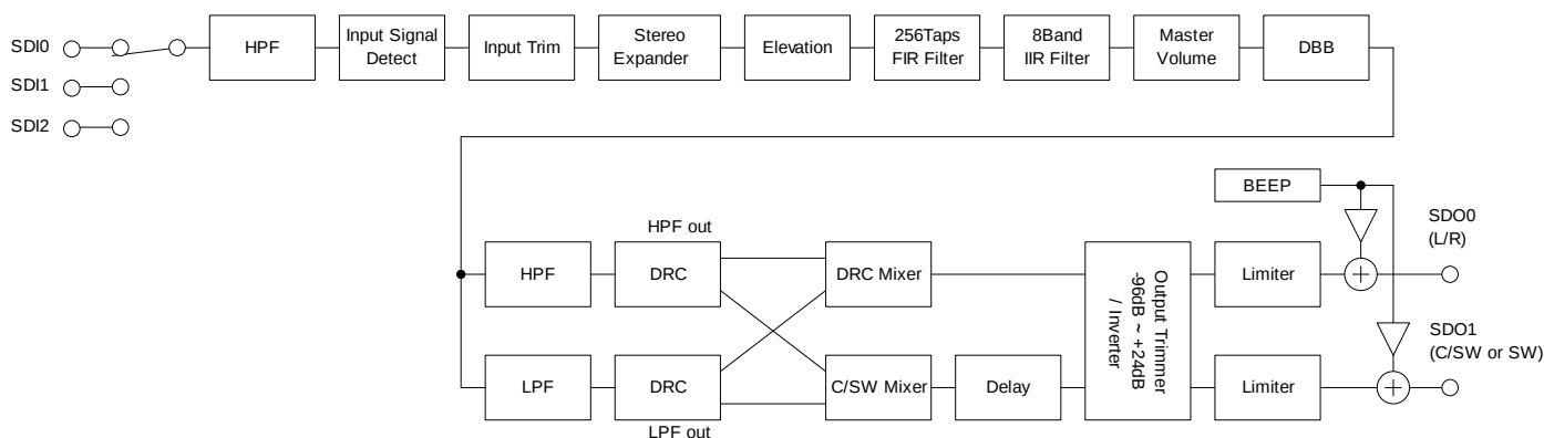
Fig 2. NJU26060-05A Block Diagram
