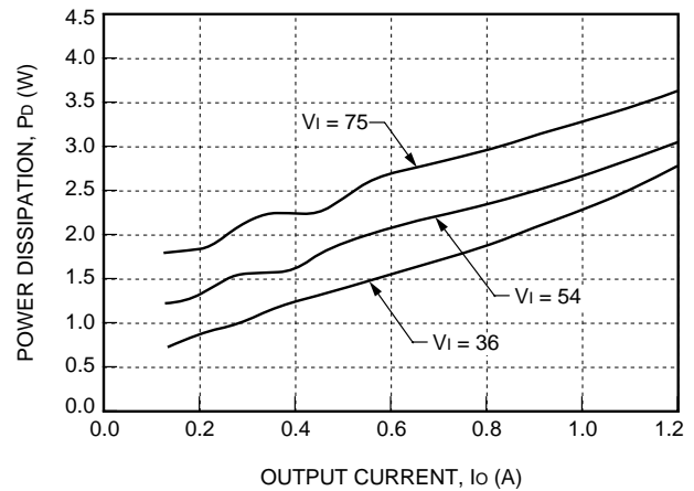
Figure 20. LW020C Power Dissipation vs. Output Current, T_A = 25\text{ }^\circ\text{C}
