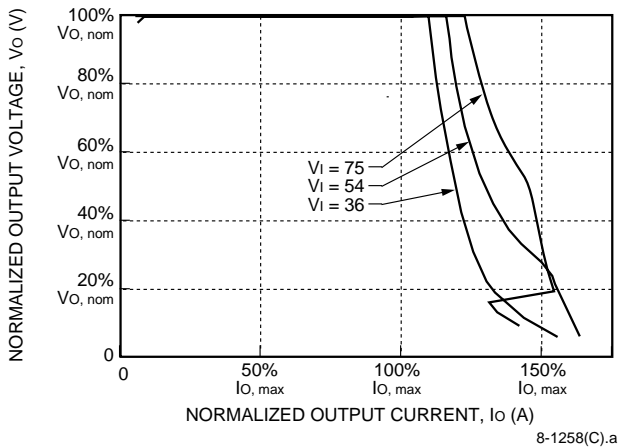
Figure 2. LW020A, B, C, F, and G Typical Output Characteristics, T_A = 25\text{ }^\circ\text{C}
