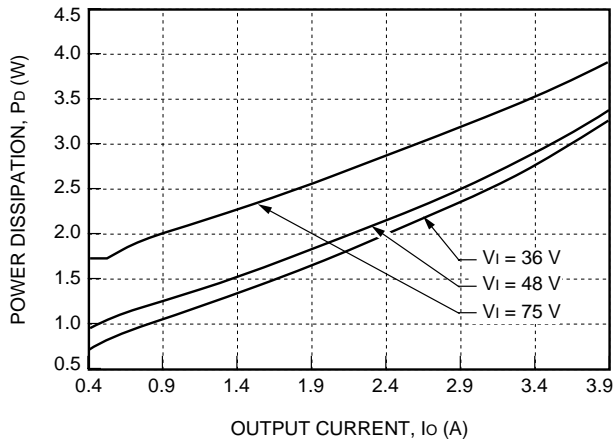
Figure 17. LW020F and G Power Dissipation vs. Output Current, T_A = 25\text{ }^\circ\text{C}
