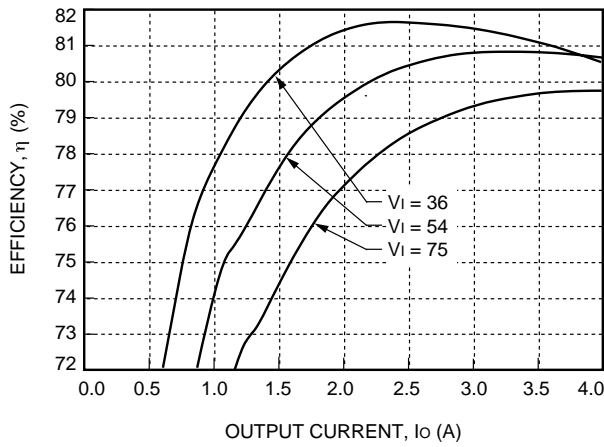
Figure 5. LW020A Typical Converter Efficiency vs. Output Current
