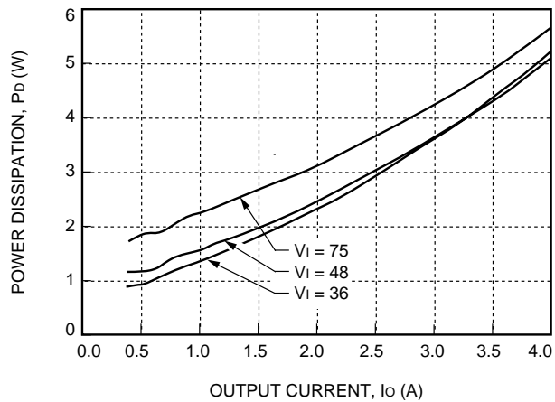
Figure 18. LW020A Power Dissipation vs. Output Current
