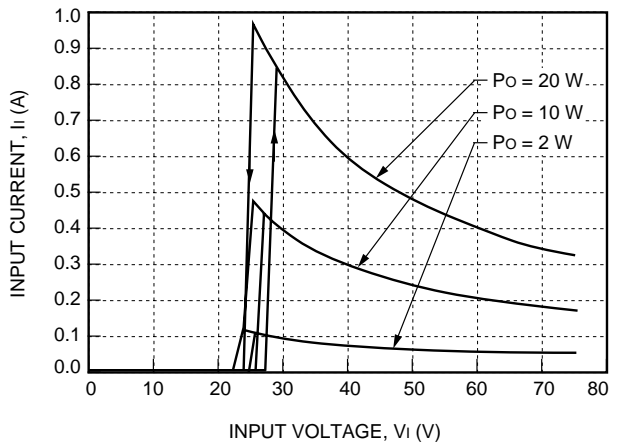
Figure 1. LW020 Typical Input Characteristics, T_A = 25\text{ }^\circ\text{C}
