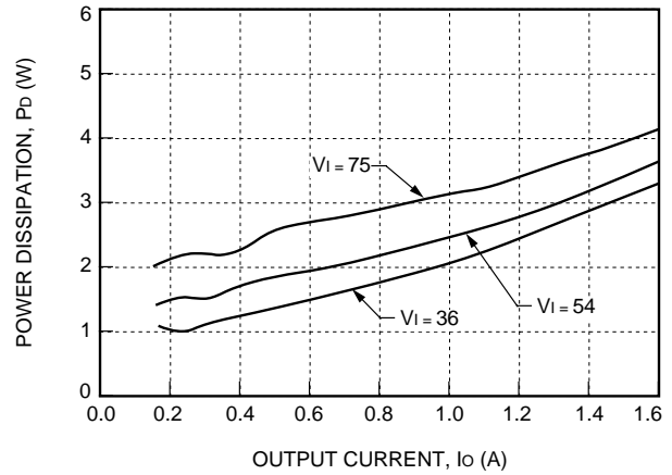
Figure 19. LW020B Power Dissipation vs. Output Current, T_A = 25\text{ }^\circ\text{C}
