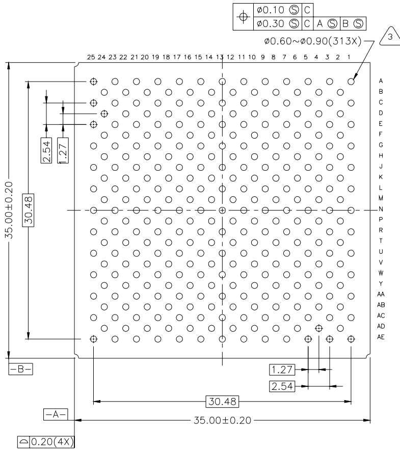
Figure 25: 313 PBGA - Bottom View
