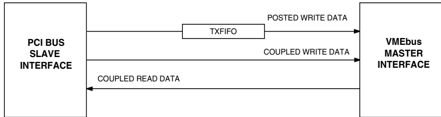
Figure 6: PCI Bus Target Channel Dataflow
