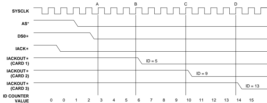
Figure 5: Timing for Auto-ID Cycle
