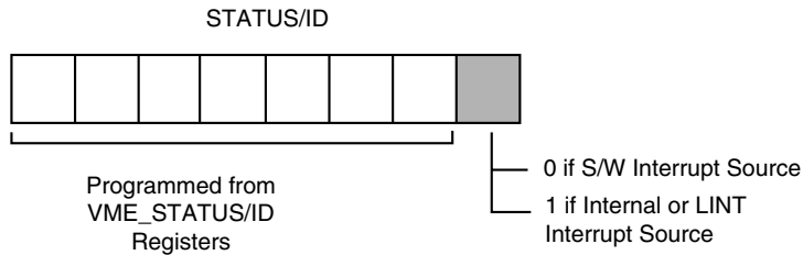
Figure 19: STATUS/ID Provided by Universe II
