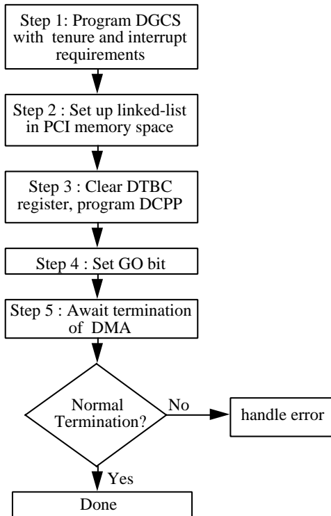
Figure 17: DMA Linked List Operation
