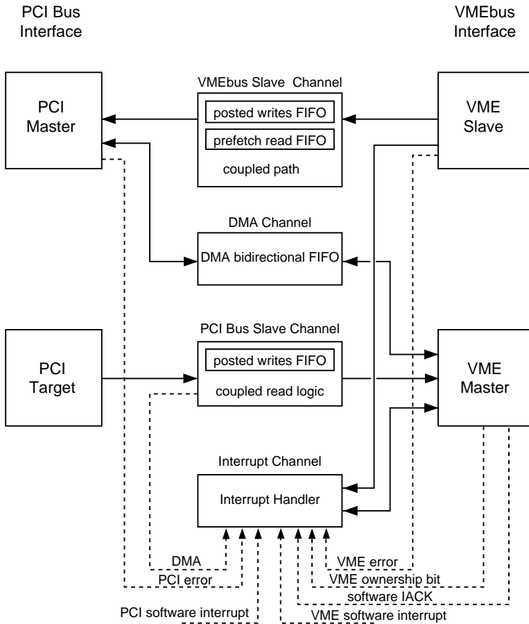
Figure 20: Sources of Internal Interrupts
