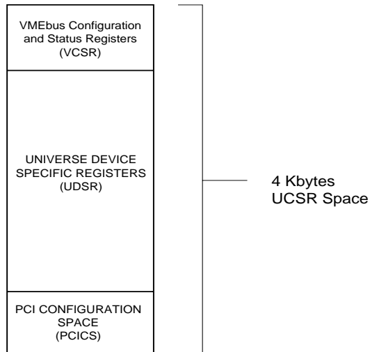
Figure 24: UCSR Access Mechanisms
