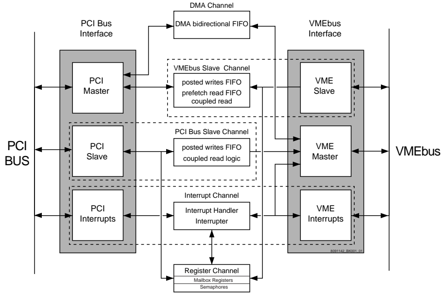
Figure 3: Universe II Data Flow Diagram
