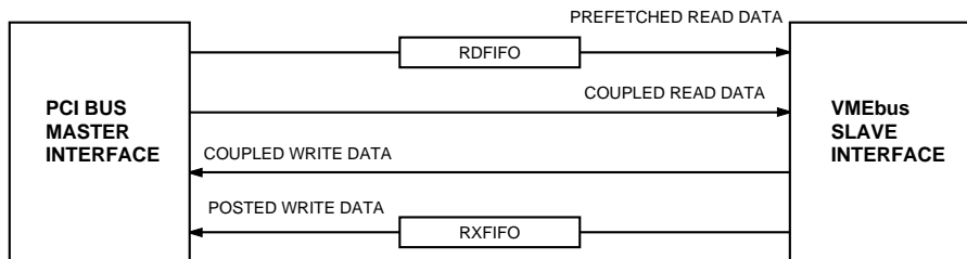
Figure 4: VMEbus Slave Channel Dataflow
