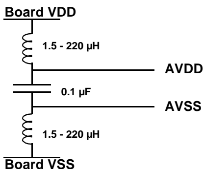
Figure 44: Analog Isolation Scheme
