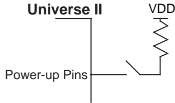
Figure 42: Power-up Configuration Using Passive Pull-ups
