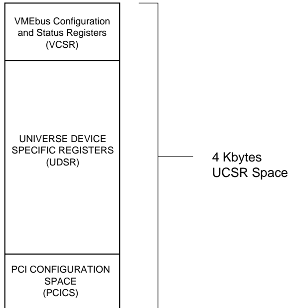
Figure 11: Universe II Control and Status Register Space
