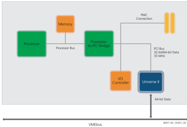
Figure 2: Universe II In Single Board Computer Application
