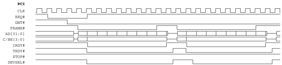
Figure 39: Multiple PCI Read Transactions During DMA Operation
