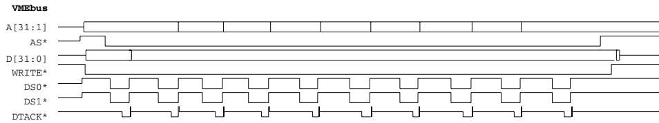
Figure 31: BLT Decoupled Write - Universe II as VME Master
