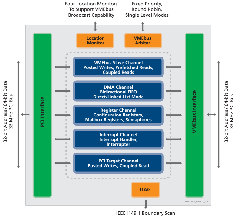
Figure 1: Universe II Block Diagram
