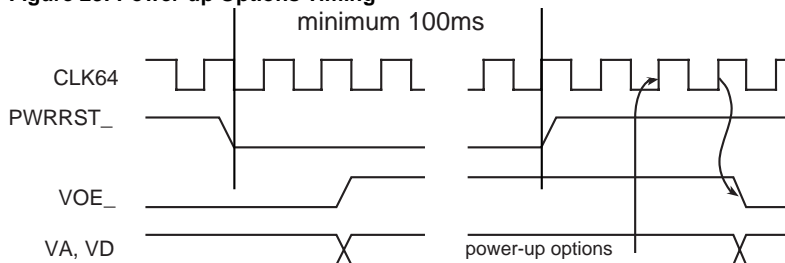
Figure 23: Power-up Options Timing
