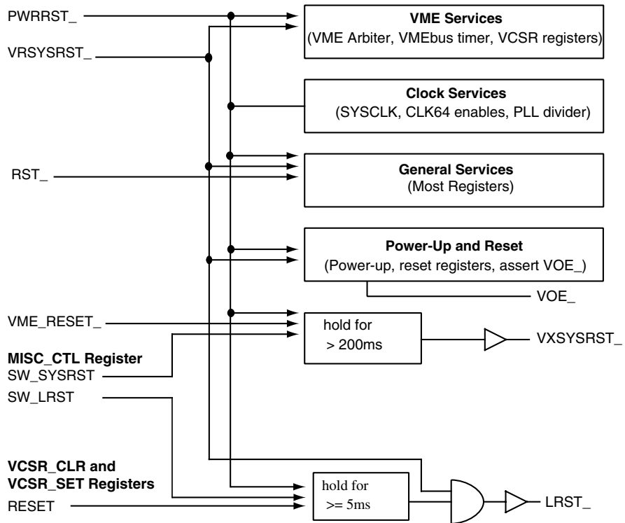
Figure 21: Reset Circuitry
