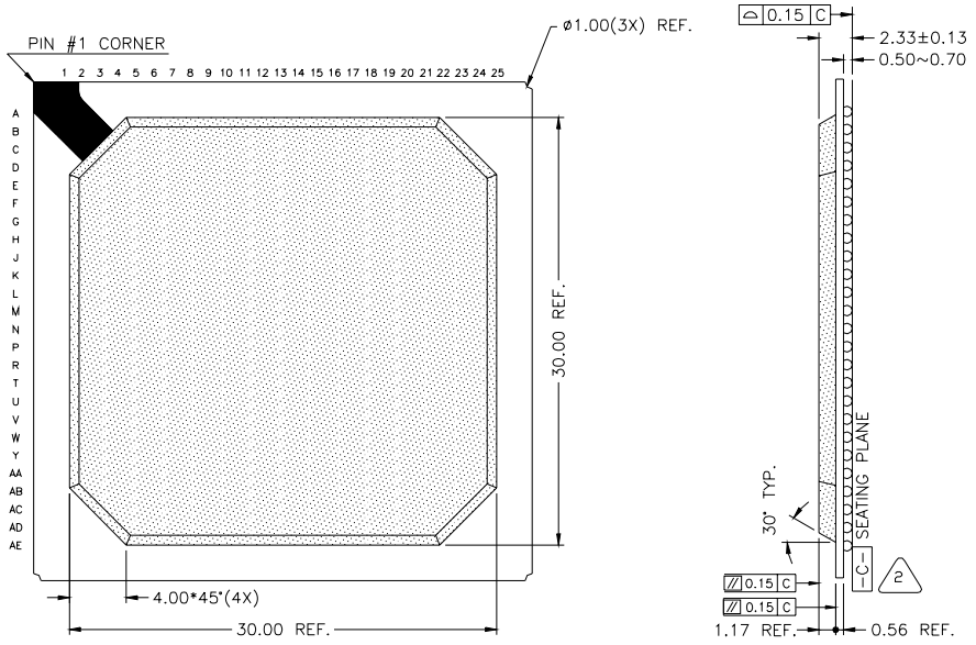
Figure 26: 313 PBGA - Top and Side View
