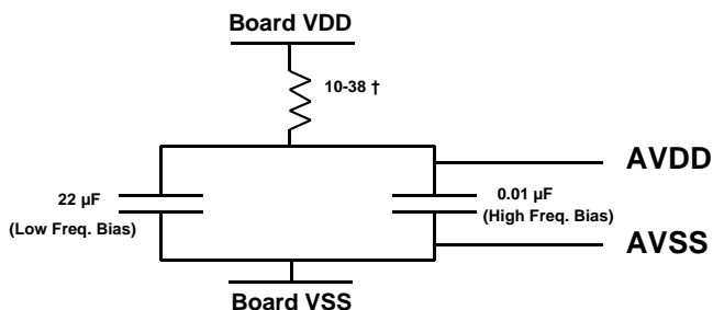
Figure 45: Noise Filter Scheme
