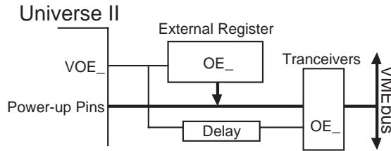
Figure 43: Power-up Configuration Using Active Circuitry
