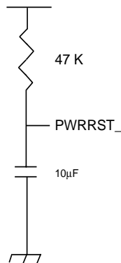
Figure 22: Resistor-Capacitor Circuit Ensuring Power-Up Reset Duration
