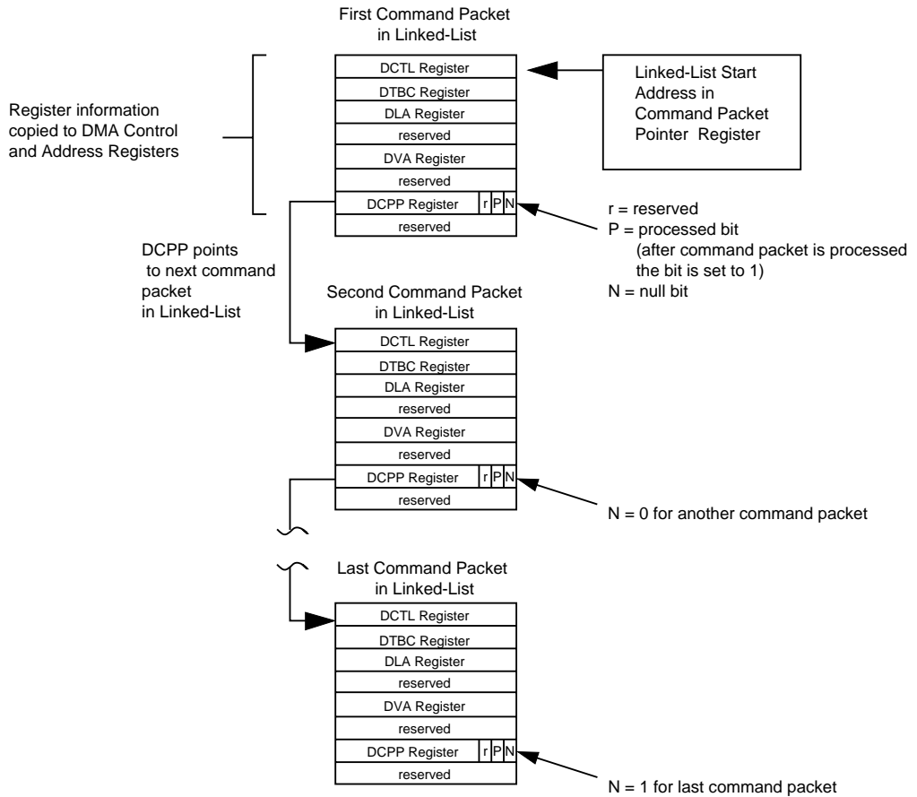
Figure 16: Command Packet Structure and Linked List Operation
