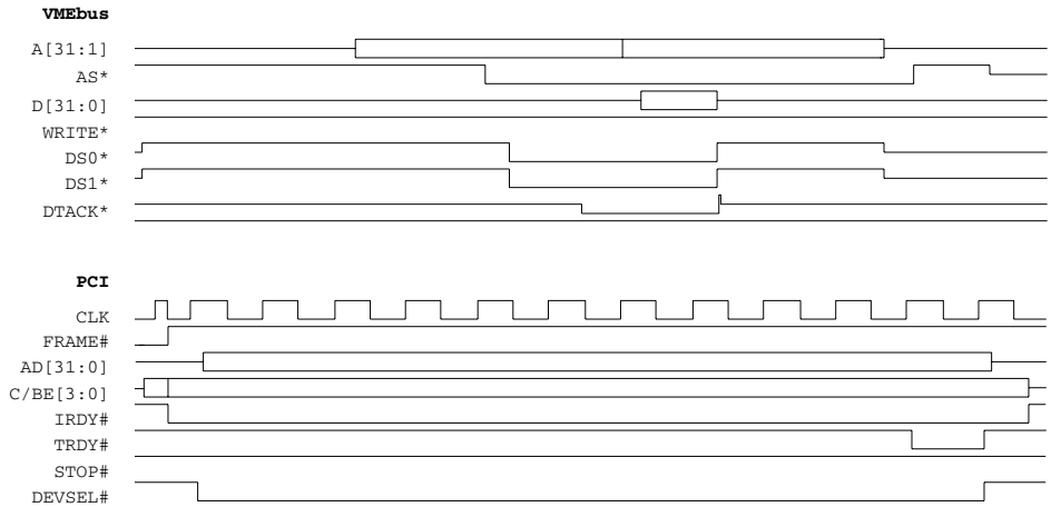
Figure 27: Coupled Read Cycle - Universe II as VME Master
