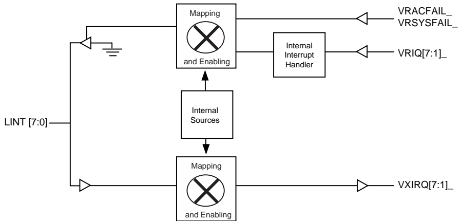
Figure 18: Universe Interrupt Circuitry
