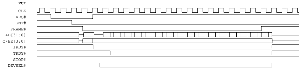
Figure 38: PCI Read Transactions During DMA Operation
