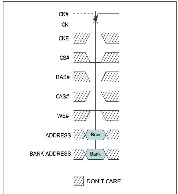
FIGURE 10 – ACTIVE COMMAND
