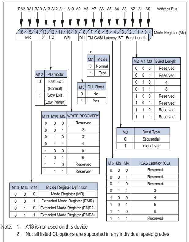
FIGURE 5 – MODE REGISTER (MR) DEFINITION
