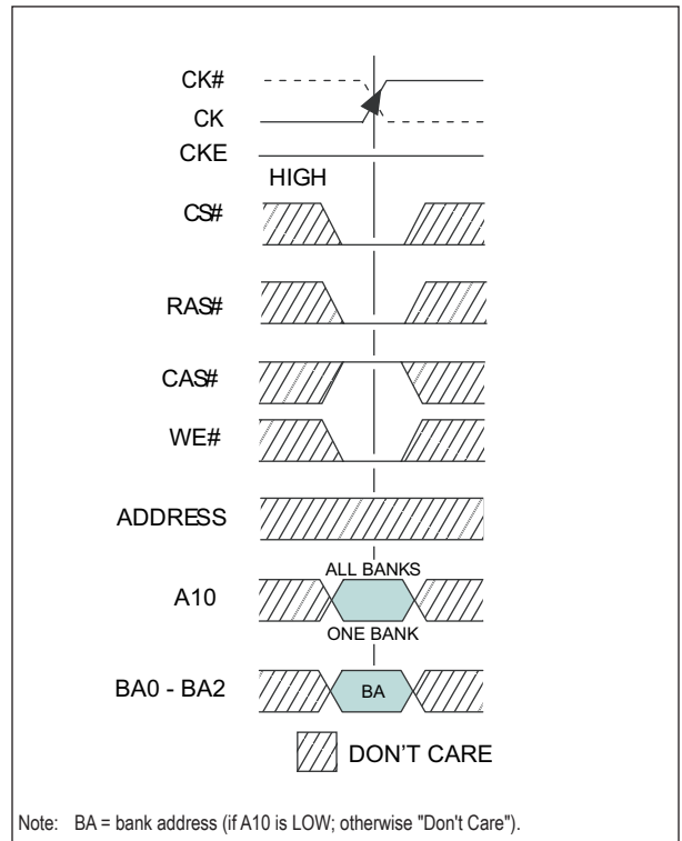
FIGURE 13 – PRECHARGE COMMAND
