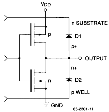
Figure 6. Equivalent Output Circuit
