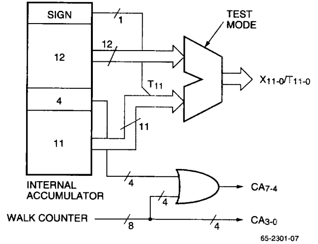
Figure 3. Test Mode Data Routing
