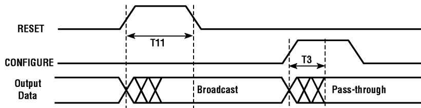
Figure 5. Reset Timing
