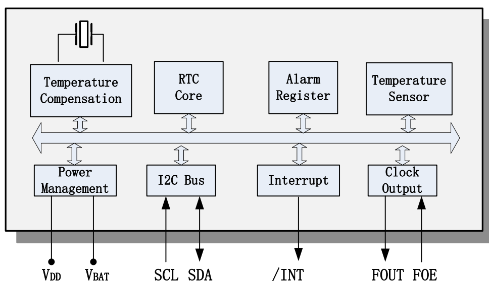
Figure 1. Block Diagram
