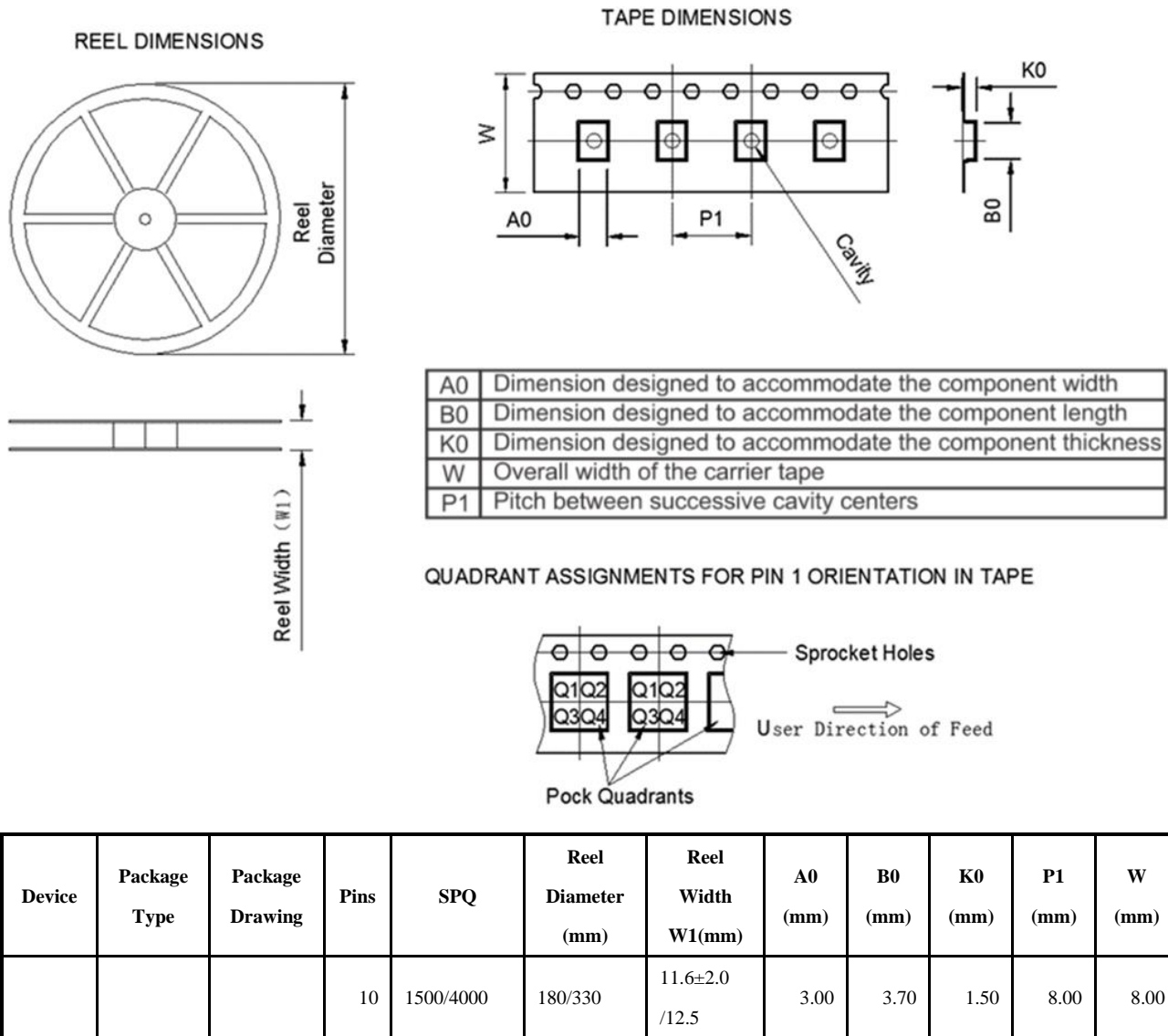
Figure 5. Package
