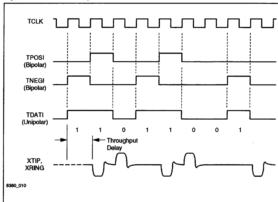
Figure 2-5. Transmitter Signals
