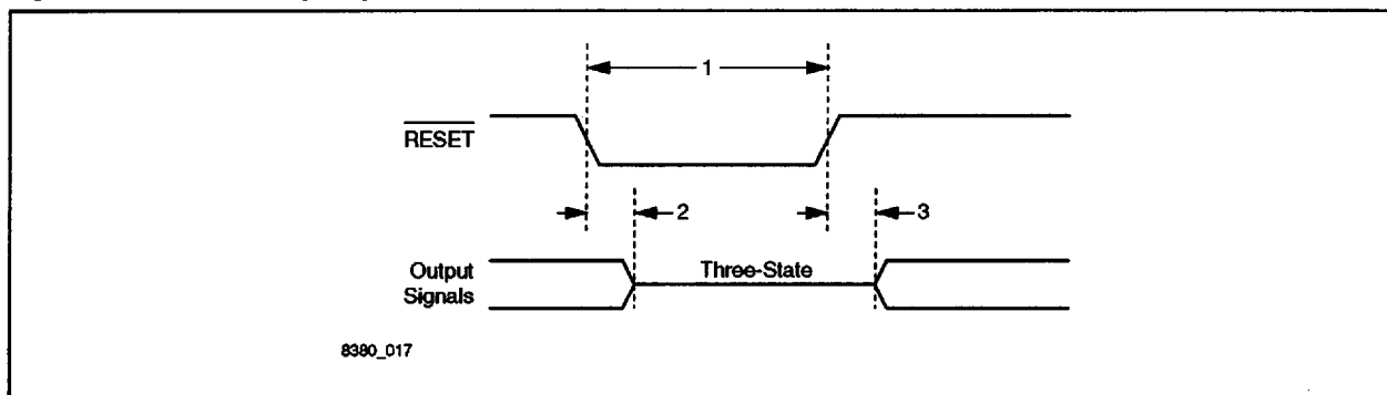
Figure 4-2. \overline{RESET} Timing Diagram
