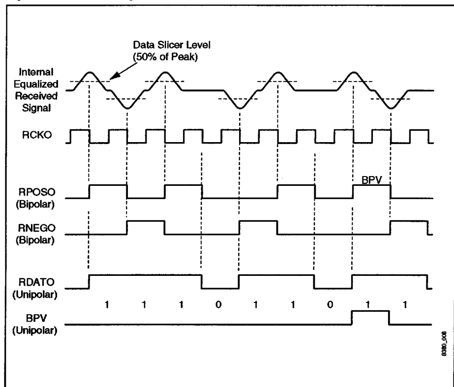
Figure 2-3. Receiver Signals
