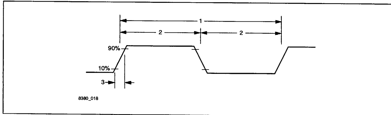
Figure 4-3. CLAD Timing Diagram
