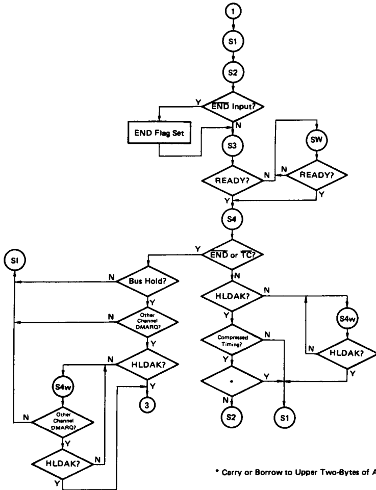
Figure 14. DMA Cycle, Block Mode
