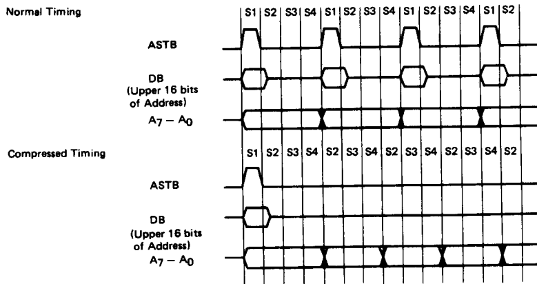
Figure 5. Normal and Compressed Timing Waveforms
