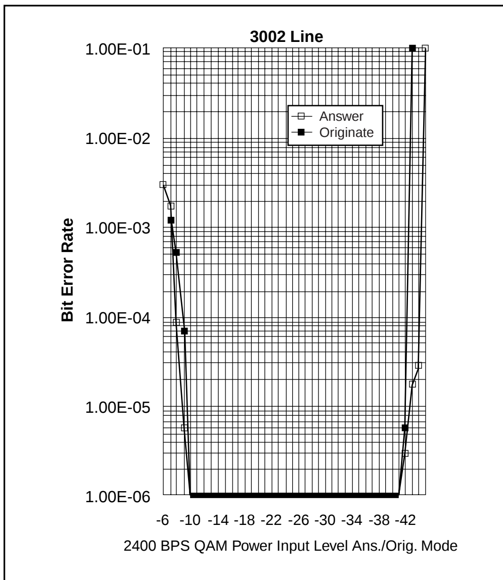
FIGURE 10 – Power Input Level vs. BER
