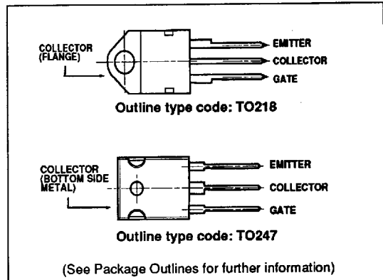
Fig. 1 Pin connections - top view (not to scale)
