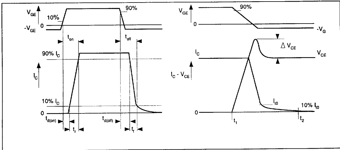
Fig.4 Definition of switching times
