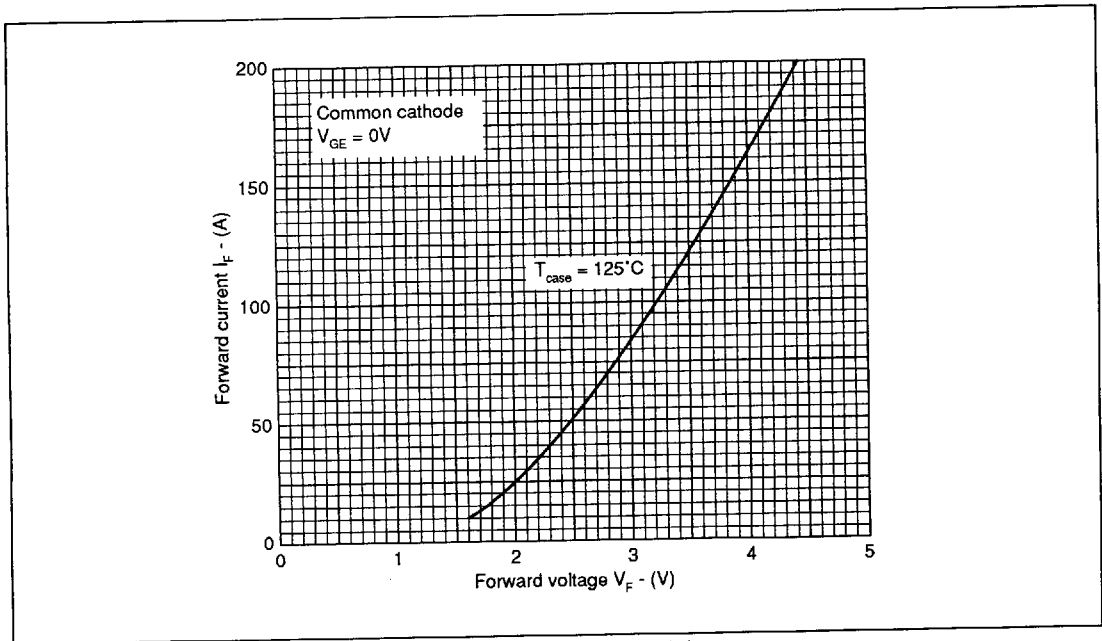
Fig. 11 Diode forward characteristics
