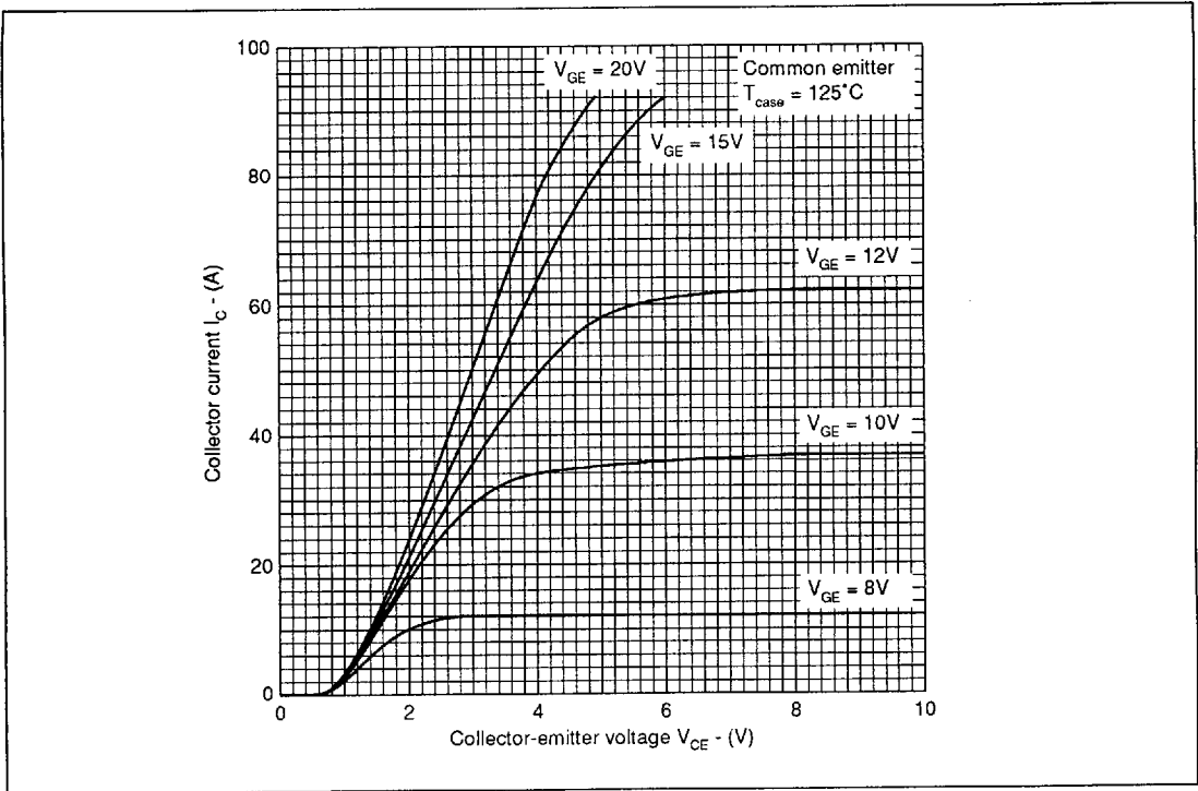
Fig.7 Typical output characteristics
