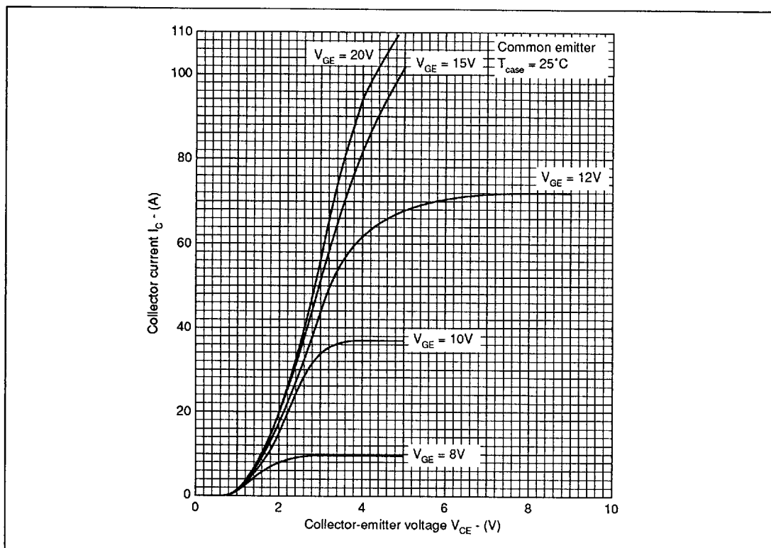
Fig.6 Typical output characteristics
