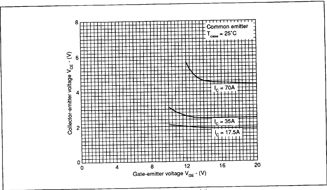
Fig. 10 Typical on-state characteristics
