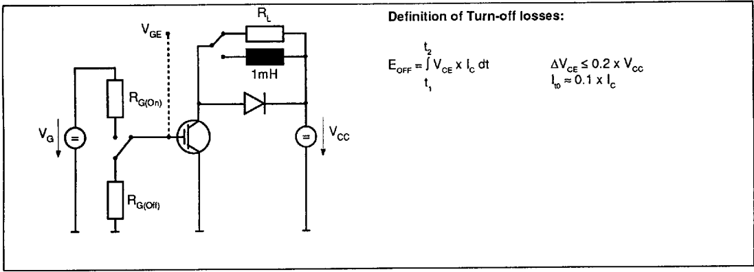
Fig.3 Test circuit
