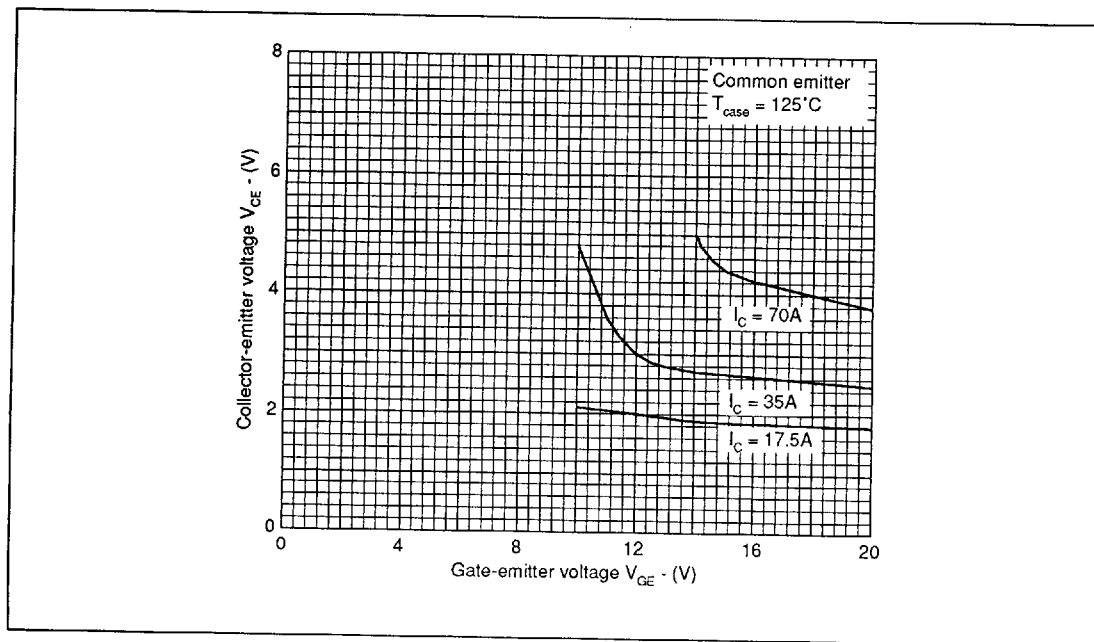
Fig.9 Typical on-state characteristics
