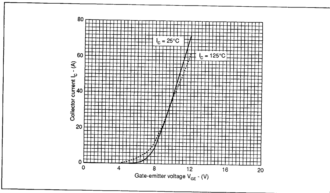
Fig.8 Typical on-state characteristics
