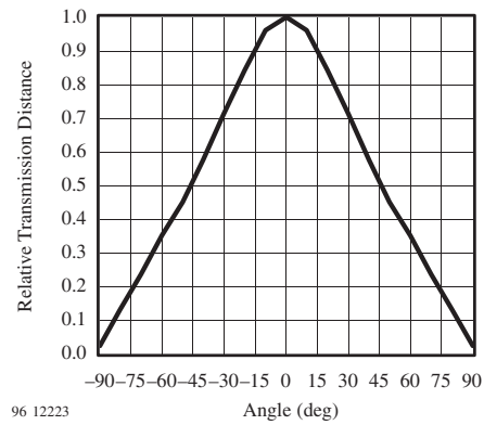
Figure 11. Directivity
