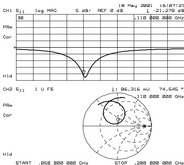
IF OUT Impedance Condition MIXER IN, LOCAL IN 50 \Omega term. V_{LNA}=V_{CONT}=0V V_{MIX}=V_{LO}=2.8V
