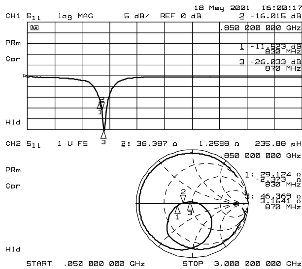
MIXER IN Impedance Condition LOCAL IN, IF OUT 50 \Omega term. V_{LNA}=V_{CONT}=0V V_{MIX}=V_{LO}=2.8V
