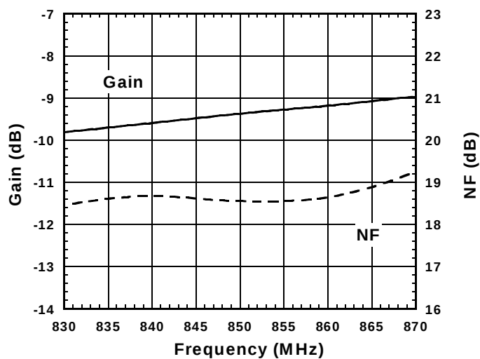
Gain, NF vs. Frequency
