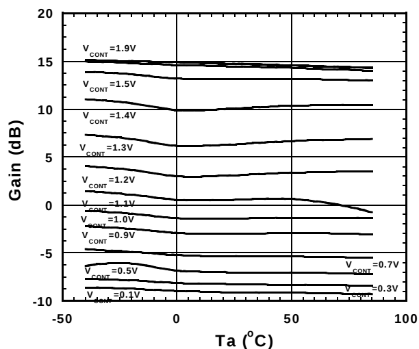
Gain vs. T_a (Variable V_{\text{CONT}} )
