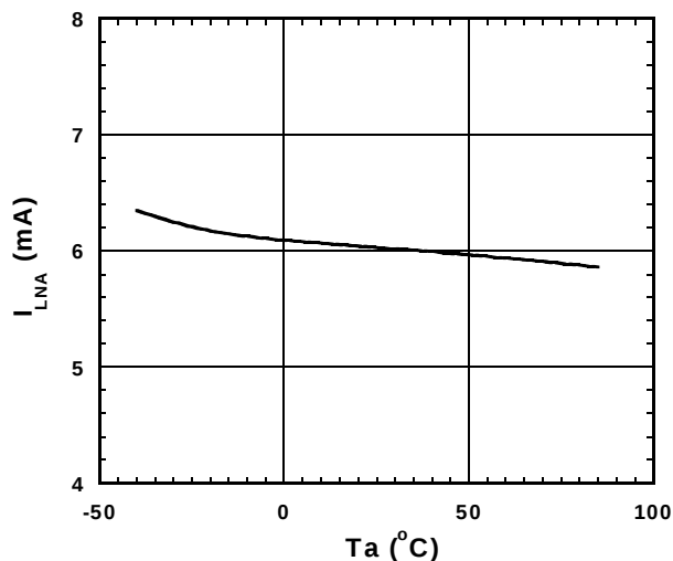
I_{\text{LNA}} vs. Ta
