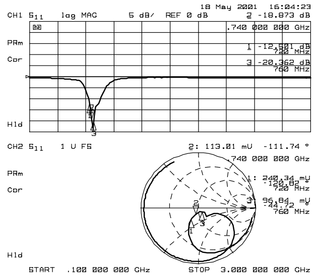
LOCAL IN Impedance Condition MIXER IN, IF OUT 50 \Omega term. V_{LNA}=V_{CONT}=0V V_{MIX}=V_{LO}=2.8V
