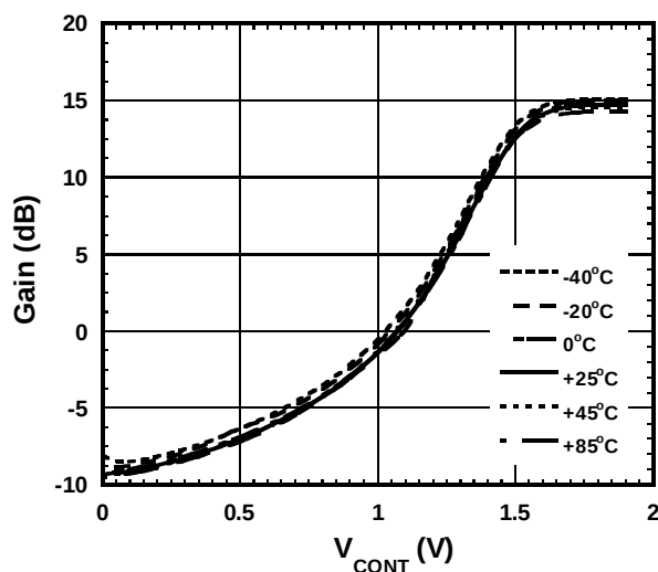
Gain vs. V_{\text{CONT}} (Variable T_a )
