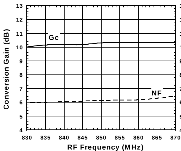
Gc, NF vs. RF Frequency
