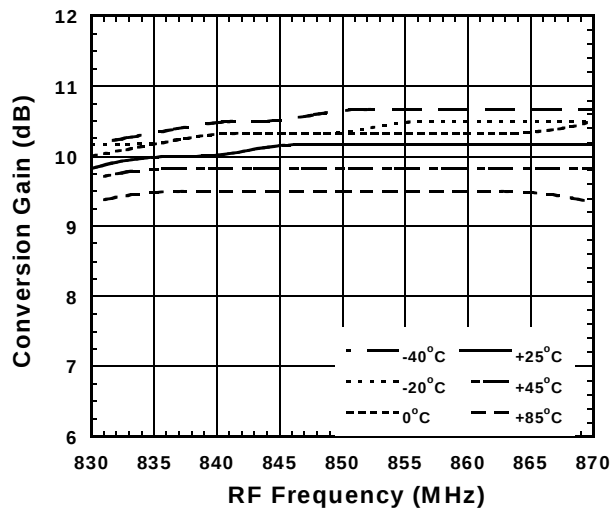
Conversion Gain vs. RF Frequency
