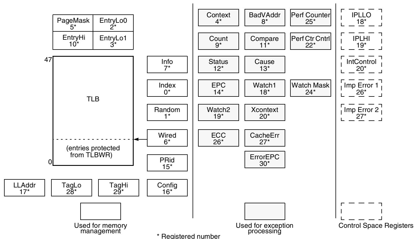
Figure 4 – CP0 Registers
