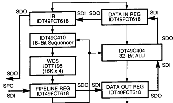
Figure 1. Typical Microprogram Application With SPC
