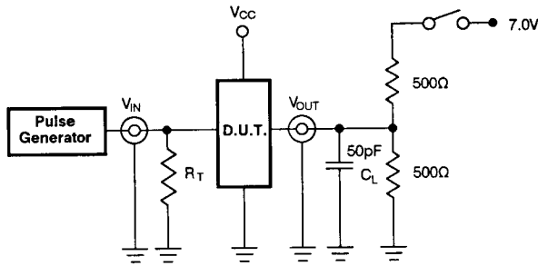
Figure 1. Switching Test Circuits (All Outputs)
