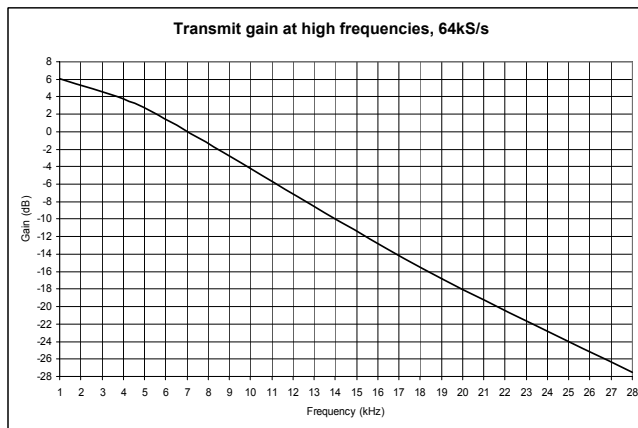
Figure 5: Transmit gain at high frequencies, 600 \Omega
