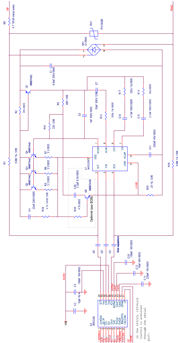
Figure 23: Application schematic
