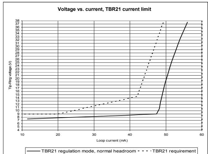
Figure 12: DC voltage versus current, TBR21 regulation
