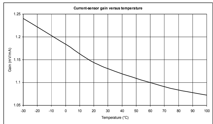
Figure 18: Current-sensor gain versus temperature s
