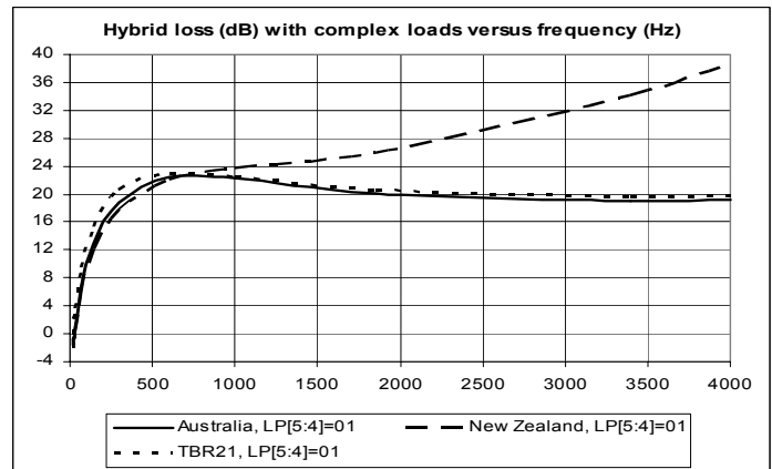
Figure 16: Trans-hybrid loss for complex modes
