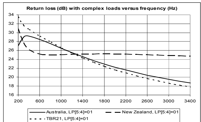
Figure 14: Return loss for complex modes
