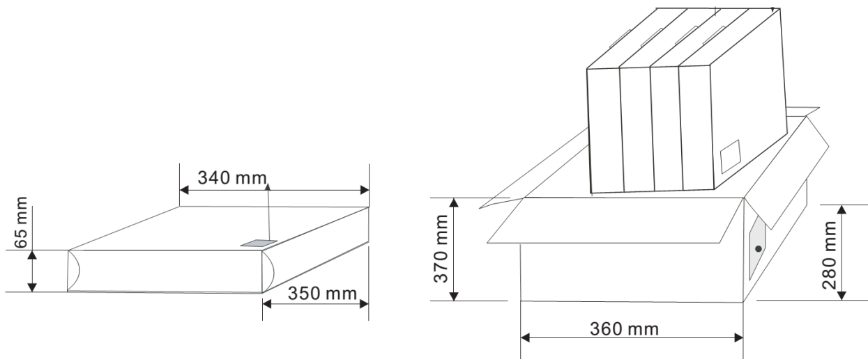
Figure 25 – Reel Cartons
