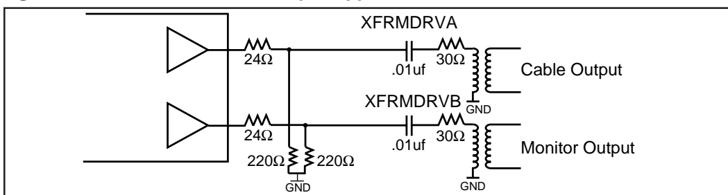
Figure 19. S3015 Transformer Output Application
