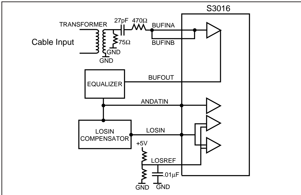
Figure 18. S3015 Differential ECL Output Application
