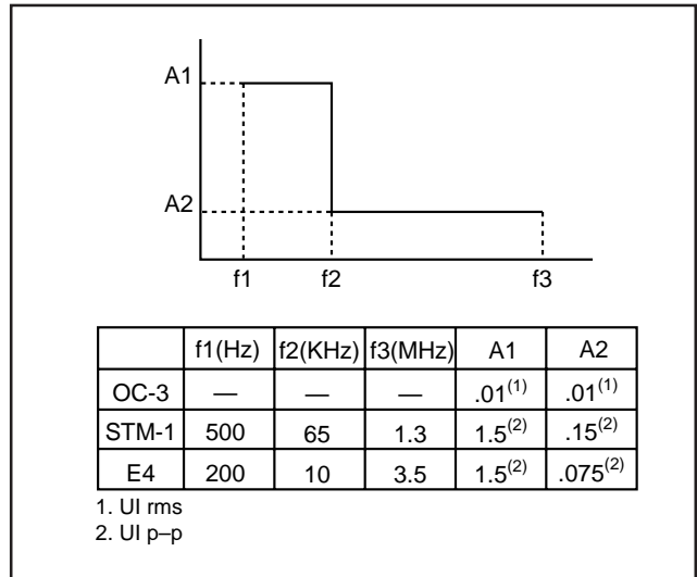
Figure 7. S3015 Maximum Allowable Input Jitter
