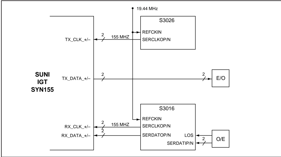
Figure 20. OC3 Application
