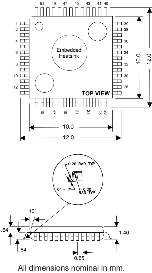
Figure 15. 52-Pin PQFP Package and Heatsink
