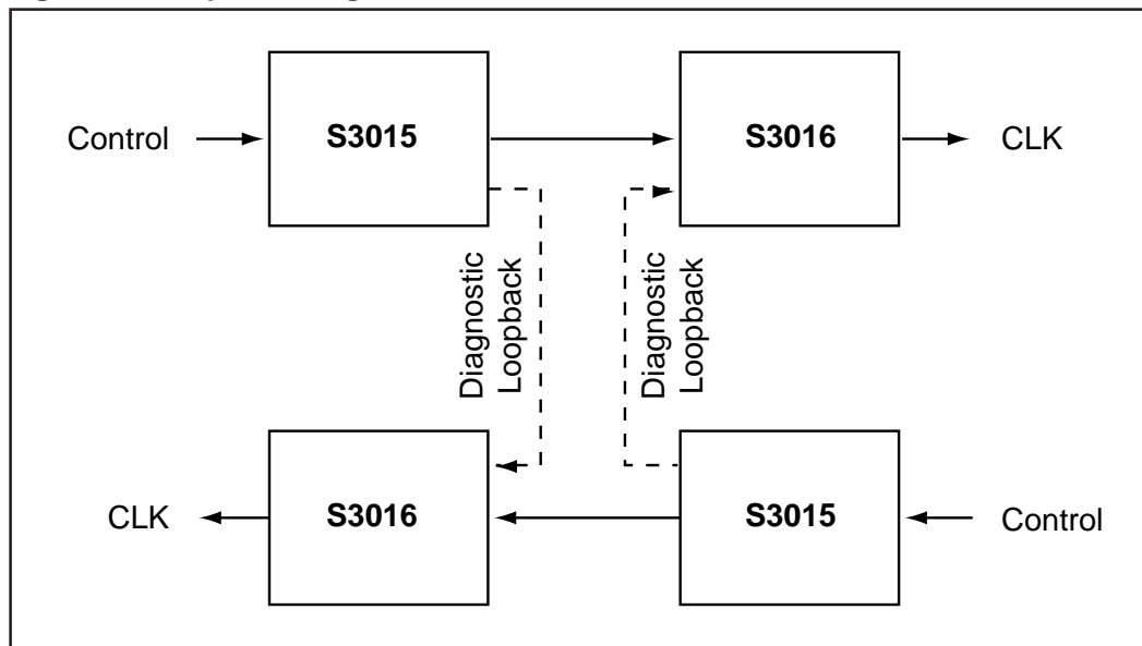
Figure 14. Loopback Diagram
