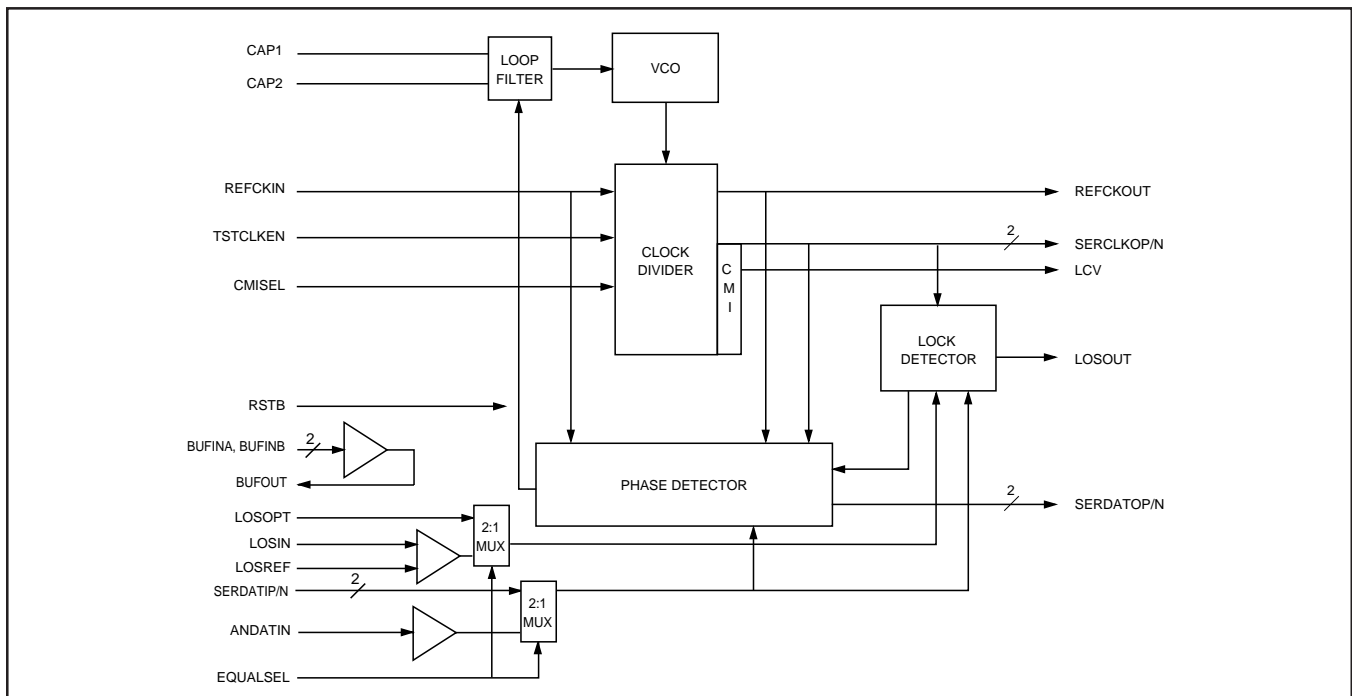
Figure 10. S3016 OC-3/STM-1/E4 Receiver Functional Block Diagram
