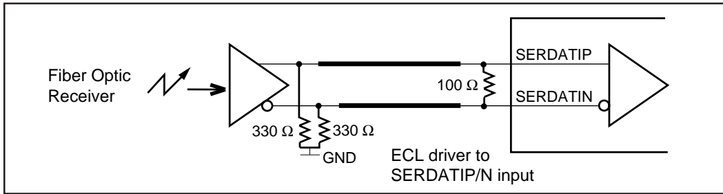
Figure 17. S3016 Transformer Input Application
