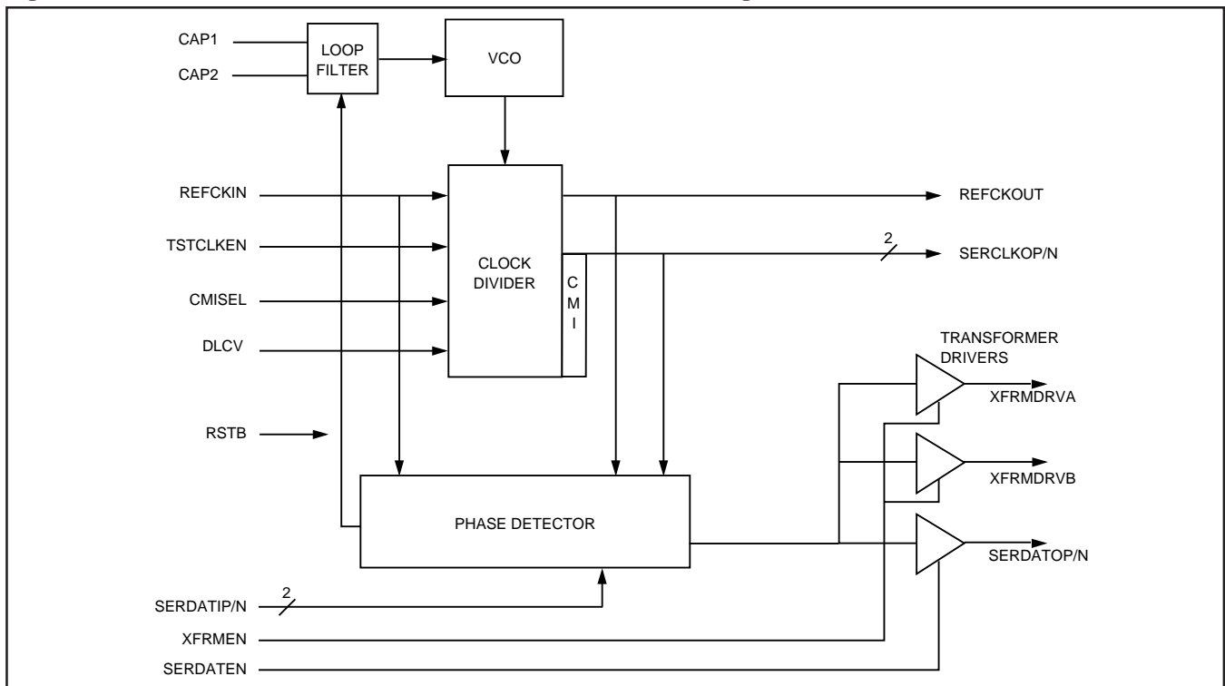
Figure 4. S3015 OC3/STM-1/E4 Transmitter Functional Block Diagram
