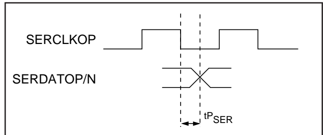
Figure 12. S3016 Clock to Data Timing
