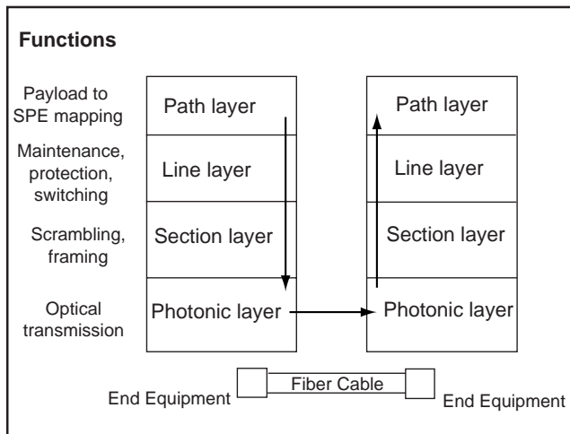
Figure 3. SONET Structure
