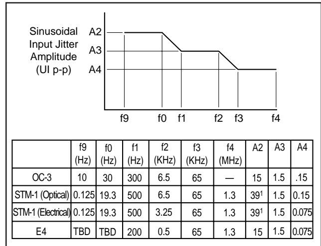
Figure 13. Clock Recovery Jitter Tolerance Compliant to G.823 and G.825
