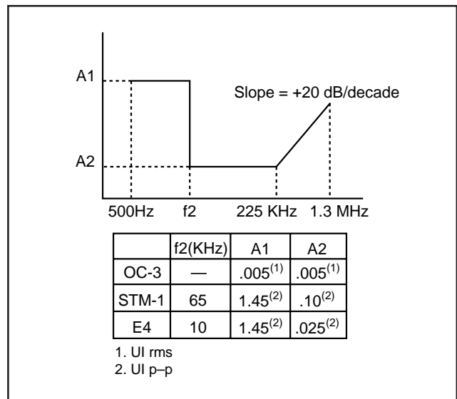
Figure 7. S3015 Maximum Allowable Input Jitter
