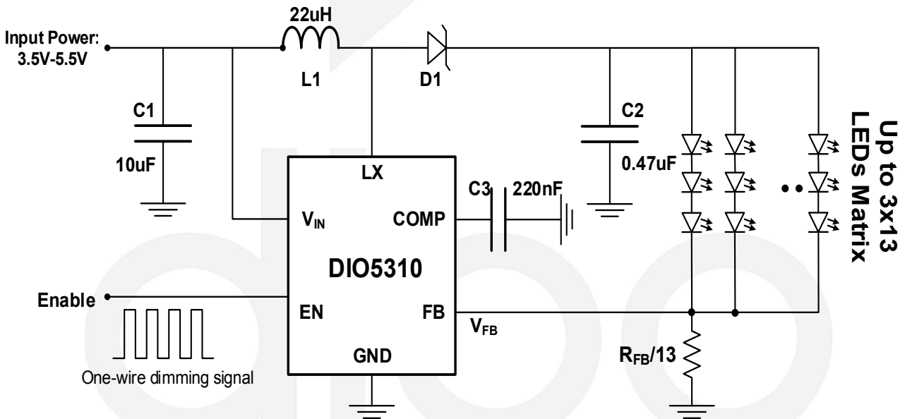
Figure 3. 3x13 (3 LEDs in row) LED Matrix Application Circuit Configuration
