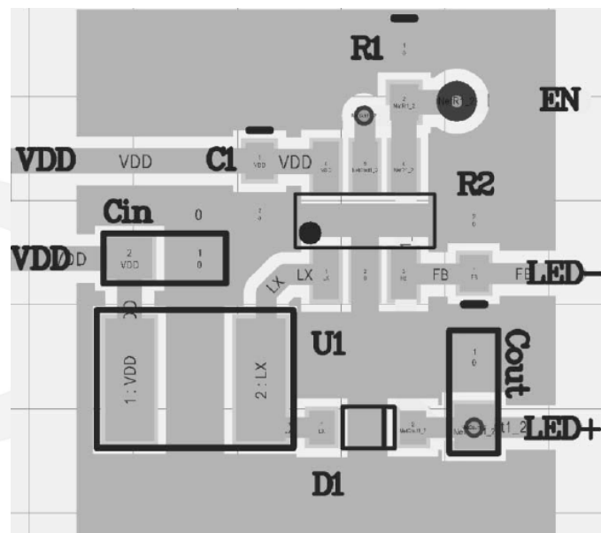
Figure 8. PCB Layout recommended
