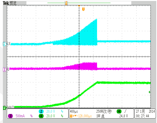
Open load at startup
