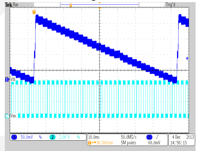
Dimming waveform
