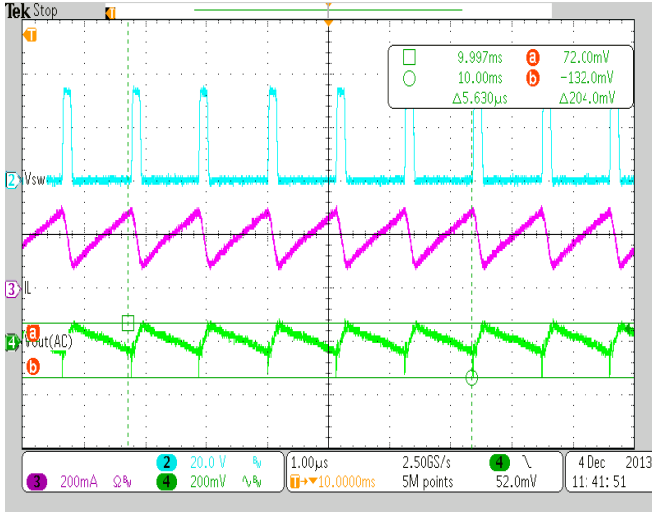
Stability waveform
