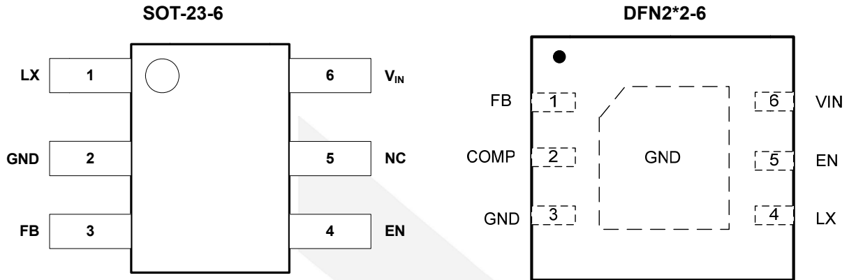
Figure 1 Top View
