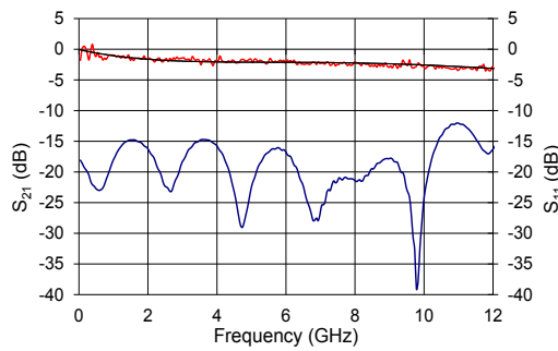
NIR-MX-LN-10: S_{21} & S_{11} Parameter Curves
