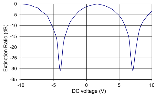
Extinction Ratio
