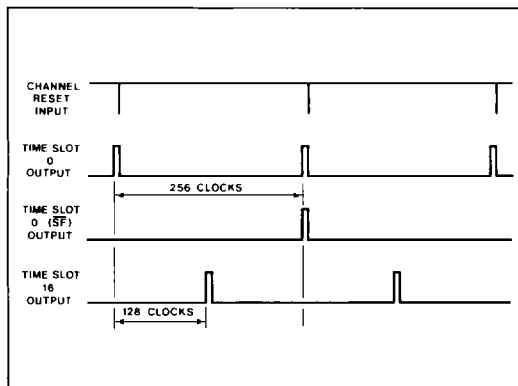
Fig.4 Sync. timing
