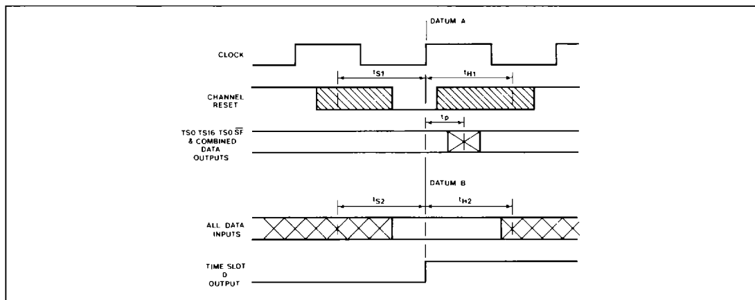
Fig.6 Timing definitions
