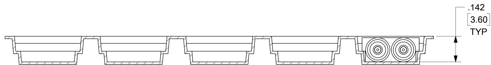
SECTION B-B
