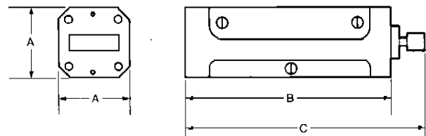
Model WR-42
