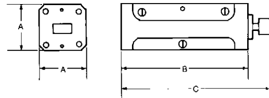
Model WR-28
