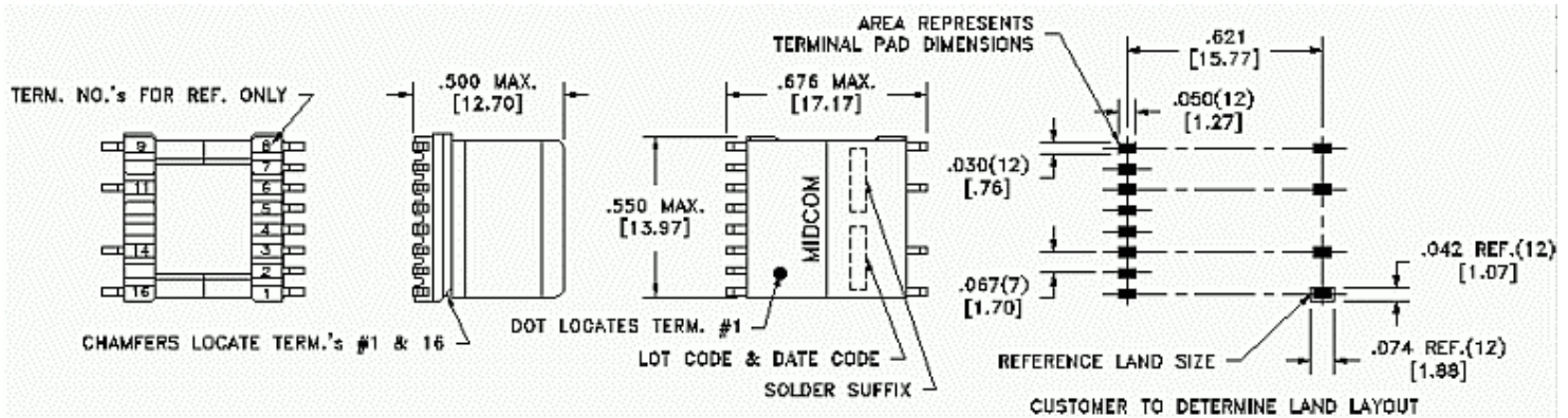
Mechanical 1
