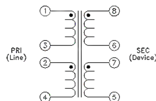
Schematic 4
