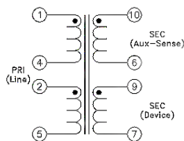
Schematic 2
