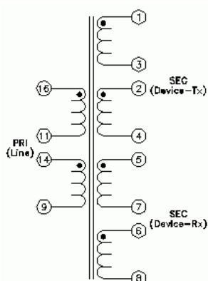
Schematic 1
