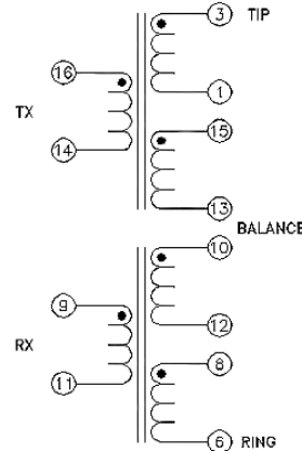
Schematic 3
