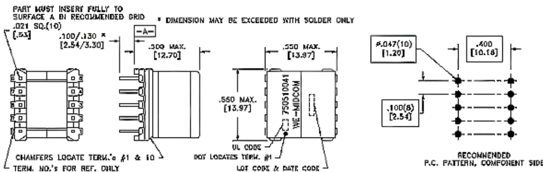
Mechanical 2
