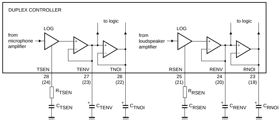
Fig.8 Signal and noise envelope detectors.
