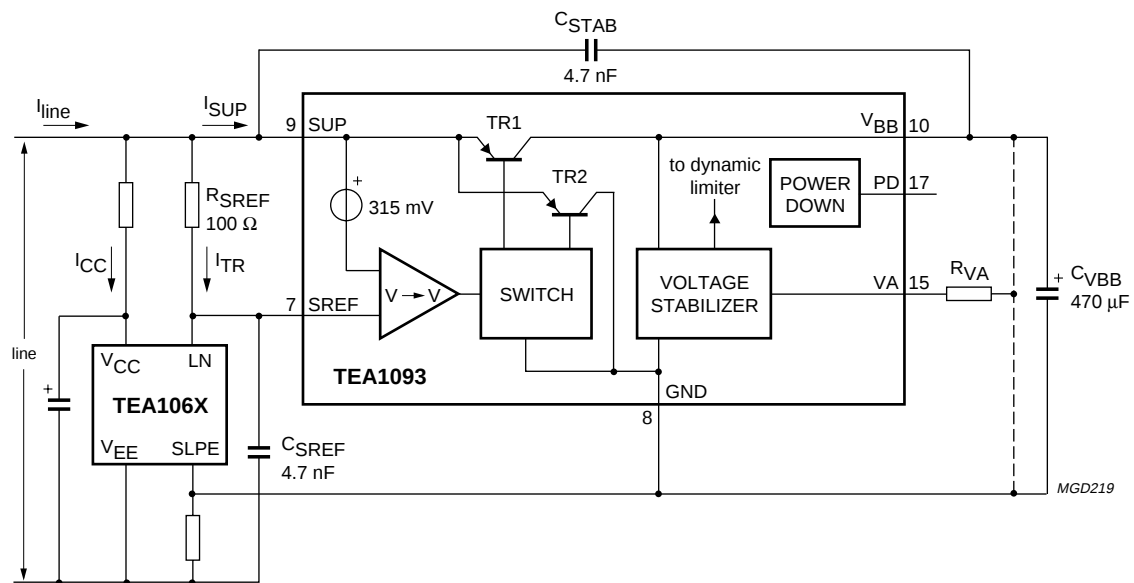
Fig.4 Supply arrangement.
