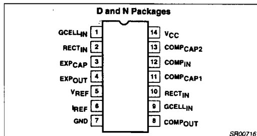
Figure 1. Pin Configuration
