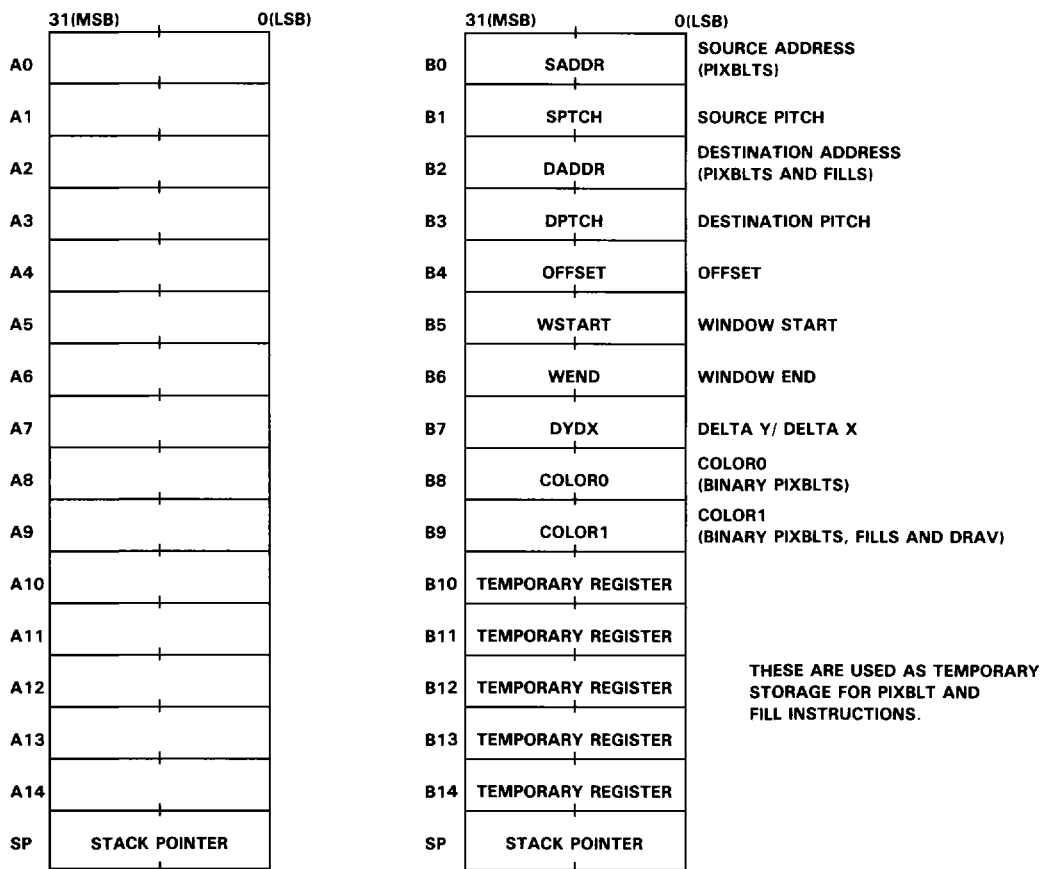
FIGURE 2. REGISTER FILES A AND B
