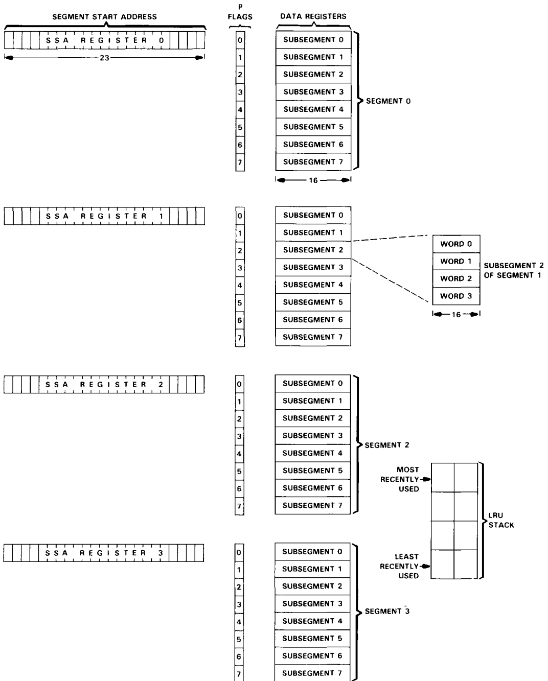
FIGURE 3. INSTRUCTION CACHE
