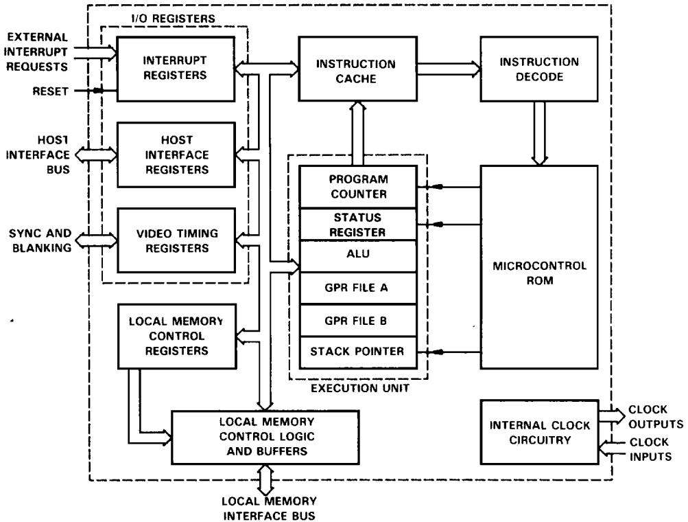
FIGURE 1. SMJ34010 INTERNAL ARCHITECTURE
