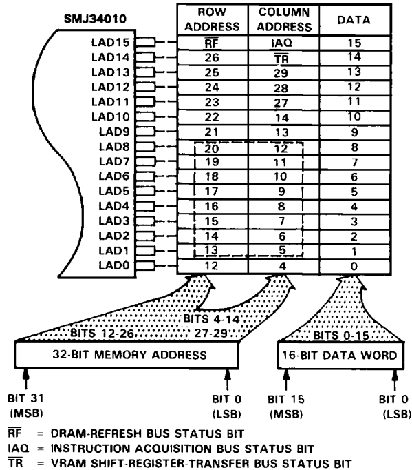
FIGURE 7. TRIPLE MULTIPLEXING OF ADDRESSES AND DATA
