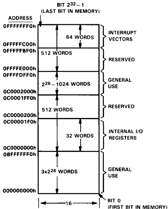
FIGURE 6. MEMORY MAP
