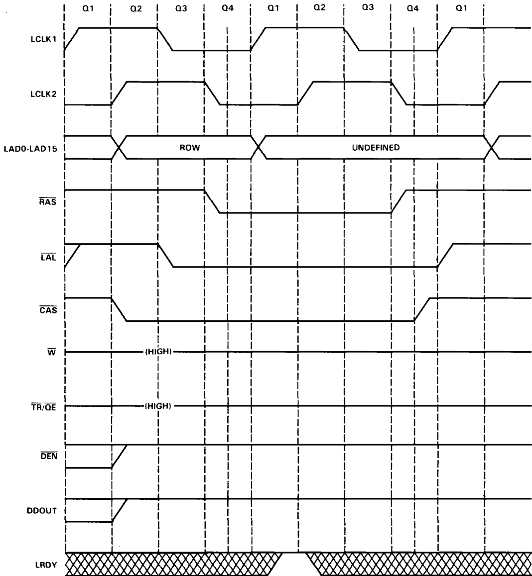
CAS-before-RAS refresh cycle timing
