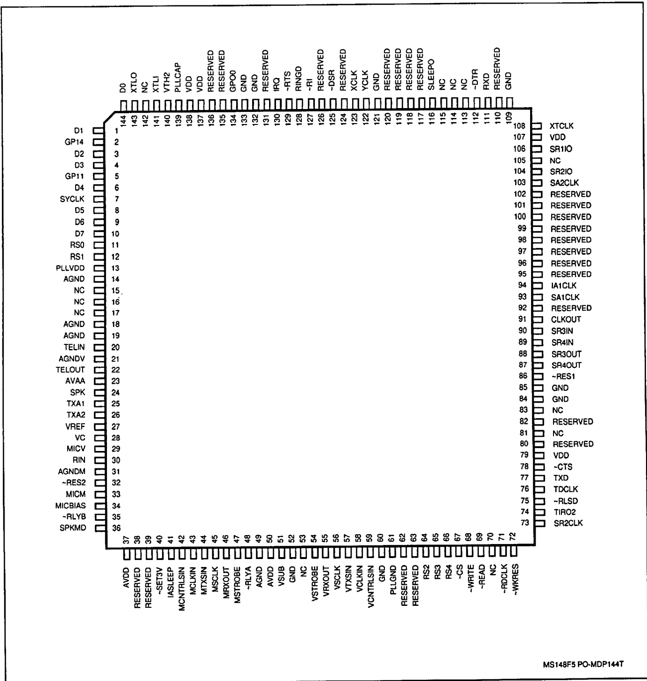
Figure 3. MDP Pin Signals - 144-Pin TQFP
