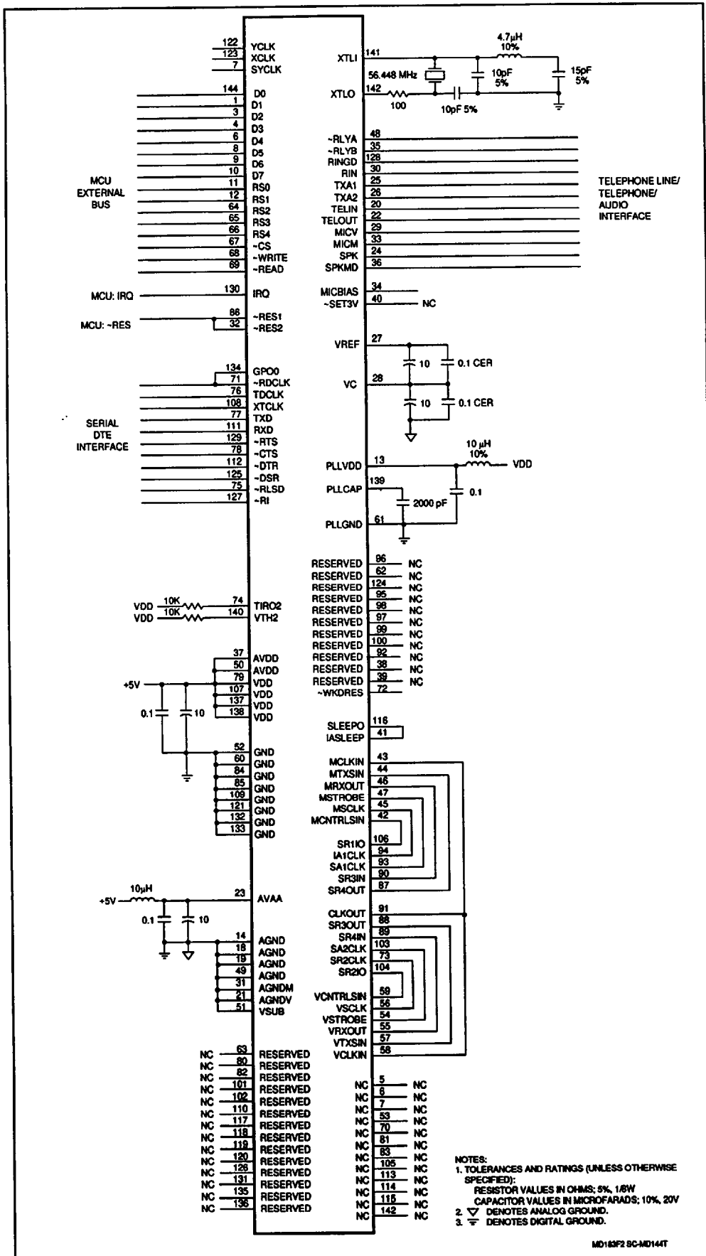
Figure 2. MDP Hardware Interface Signals-144-Pin TQFP
