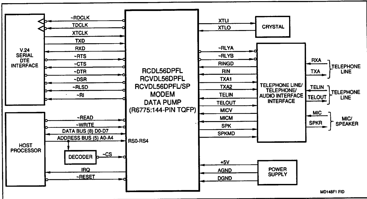
Figure 1. RCVDL56DPFL/SP MDP Functional Interface
