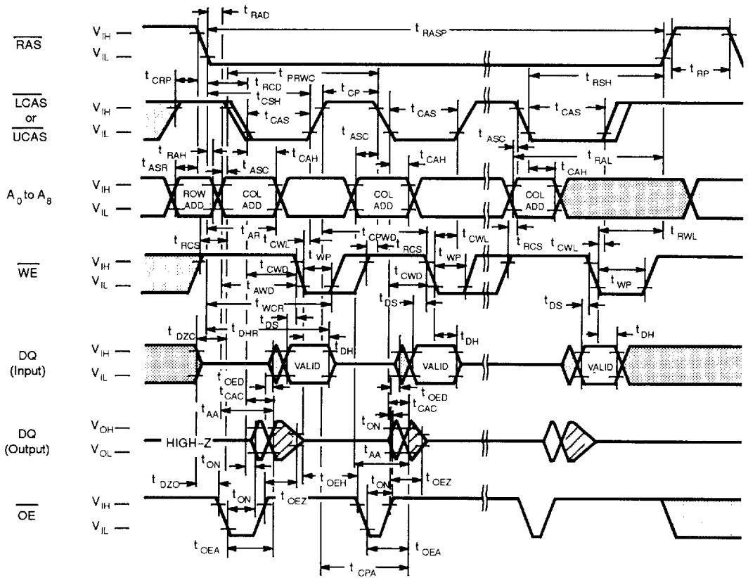
Fig. 12 - FAST PAGE MODE READ-MODIFY-WRITE CYCLE
