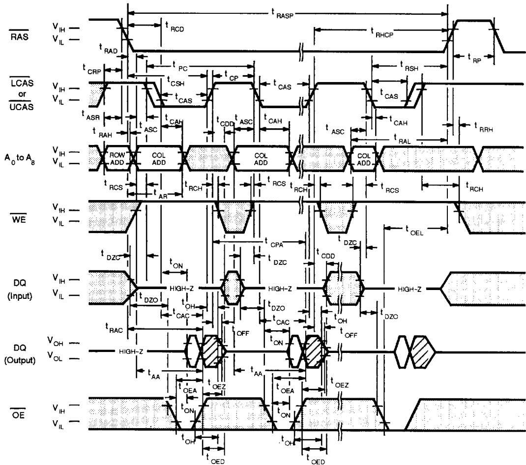
Fig. 9 - FAST PAGE MODE READ CYCLE
