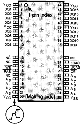
44-Pin FPT: (TOP VIEW)
