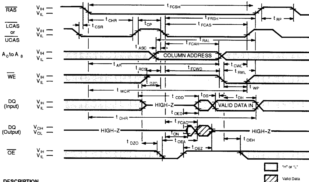
Fig. 16 - \overline{\text{CAS}} -BEFORE- \overline{\text{RAS}} REFRESH COUNTER TEST CYCLE
