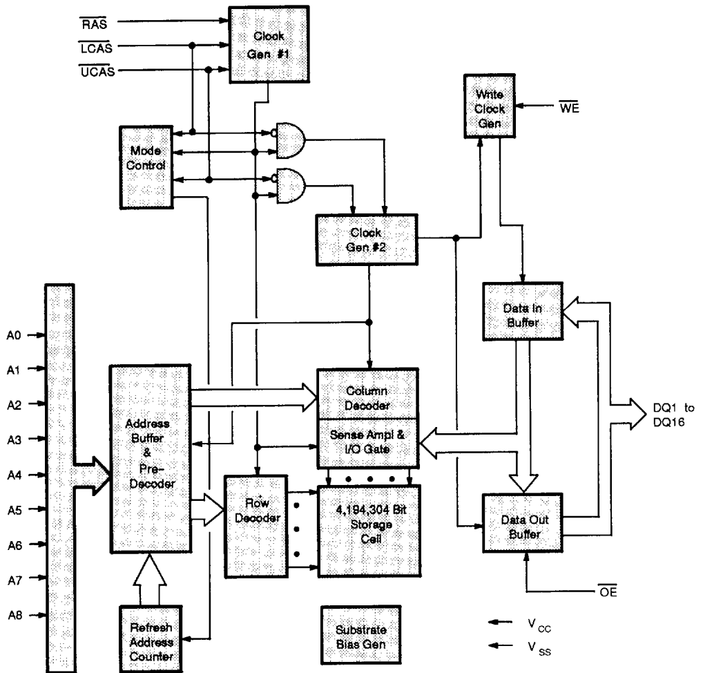
Fig. 1 - MB814260 DYNAMIC RAM - BLOCK DIAGRAM
