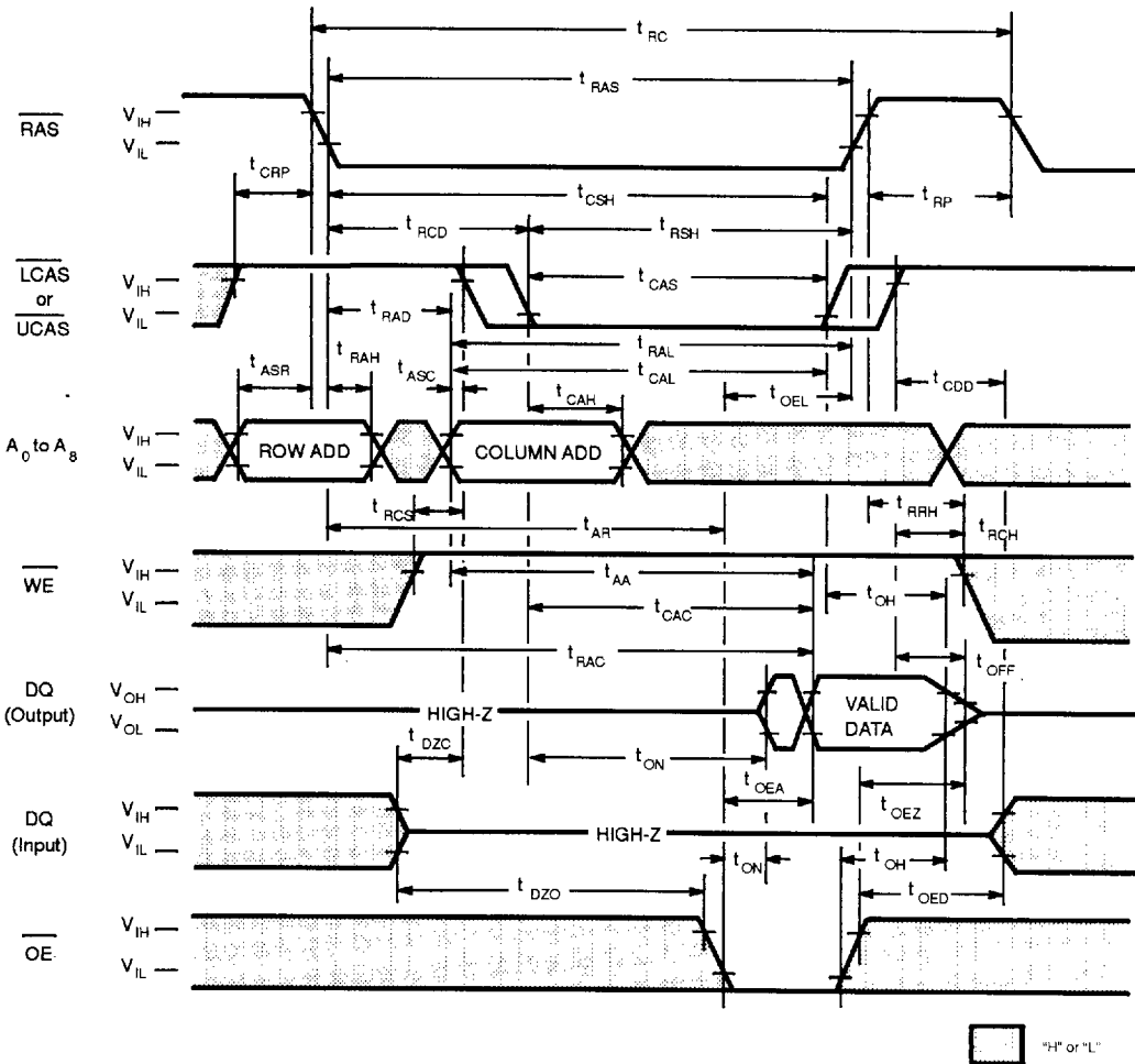
Fig. 5 - READ CYCLE
