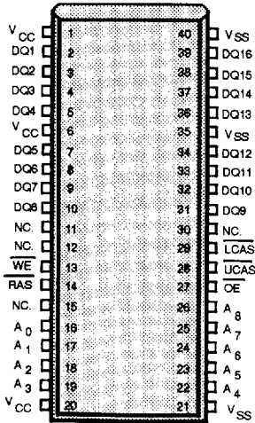
40-Pin SOJ: (TOP VIEW)
