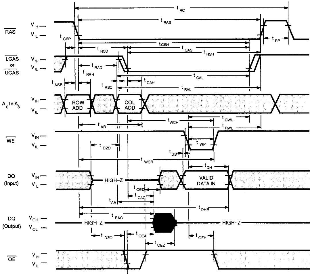
Fig. 7 - \overline{OE} (DELAYED WRITE CYCLE)
