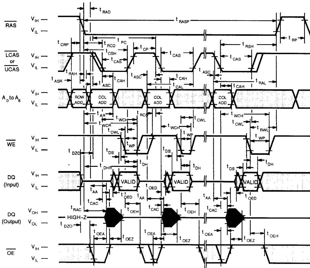
Fig. 11 - FAST PAGE MODE \overline{OE} WRITE CYCLE
