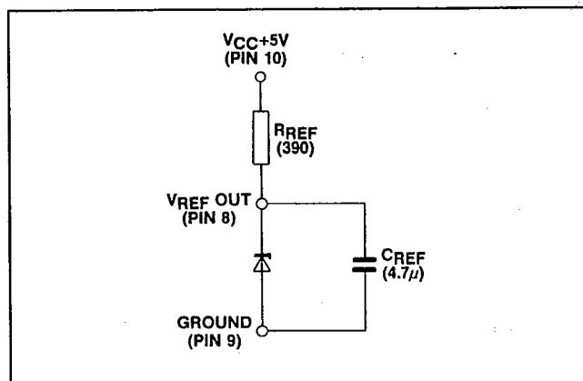
Fig. 10 Internal voltage reference
