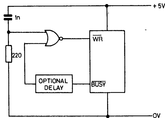
Fig. 3a Circuit for continuous conversion
