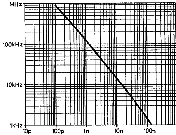
Fig. 8 Typical clock frequency v CCK (RCK = 0)
