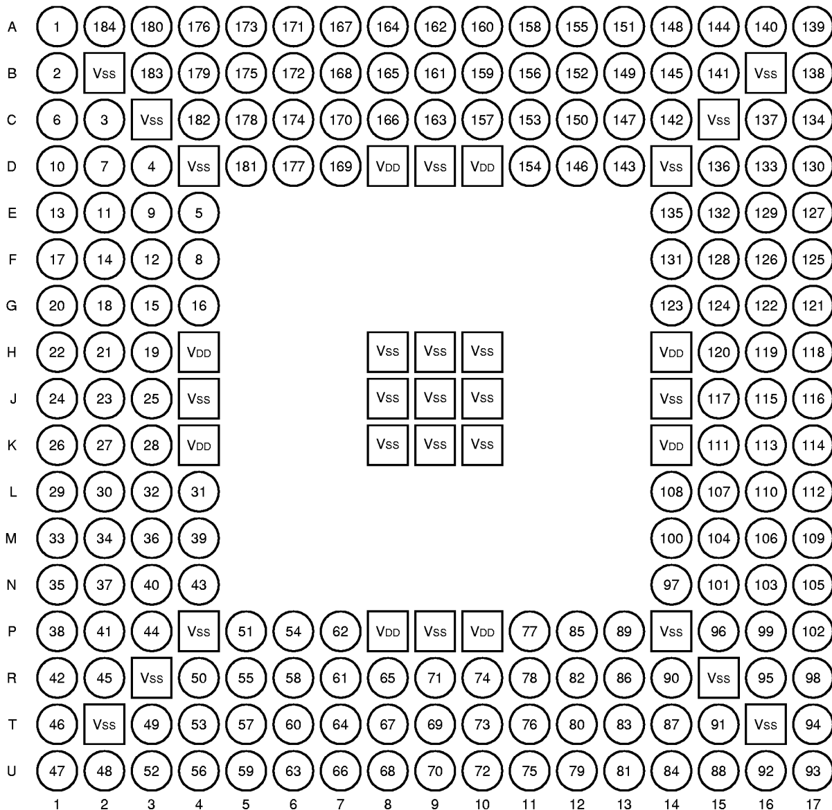
Figure 2. 217 PBGA—Top View
