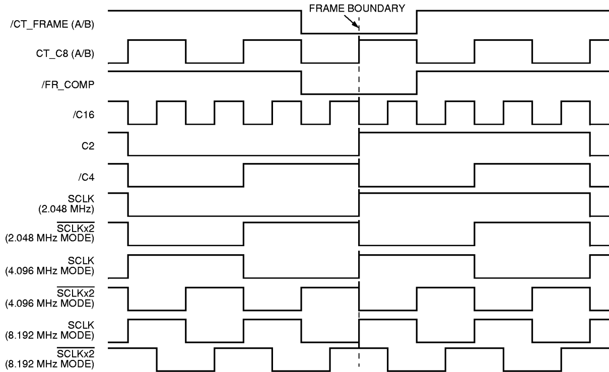
Figure 19. Clock Alignment
