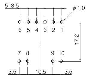
Recommended Piercing Plan (Top View)
