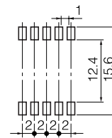
Recommended land pattern (Top View)
