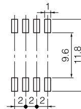
Recommended land pattern (Top View)
