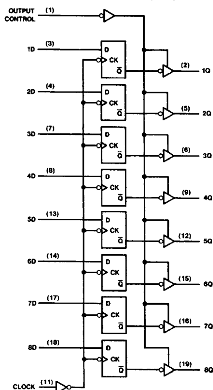
Positive-Edge-Triggered Flip-Flops
