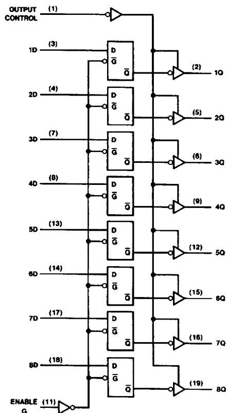
Transparent Latches
