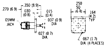
Flange Mount Jack
