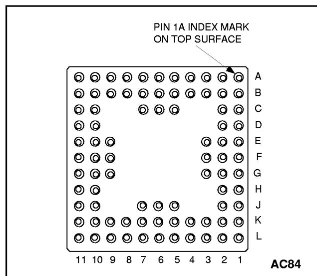
Fig.1 Pin connections - bottom view (AC84 - PGA)
