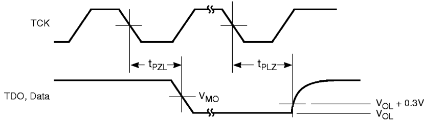
Figure 13. Tri-state Output Low, Enable and Disable Times
