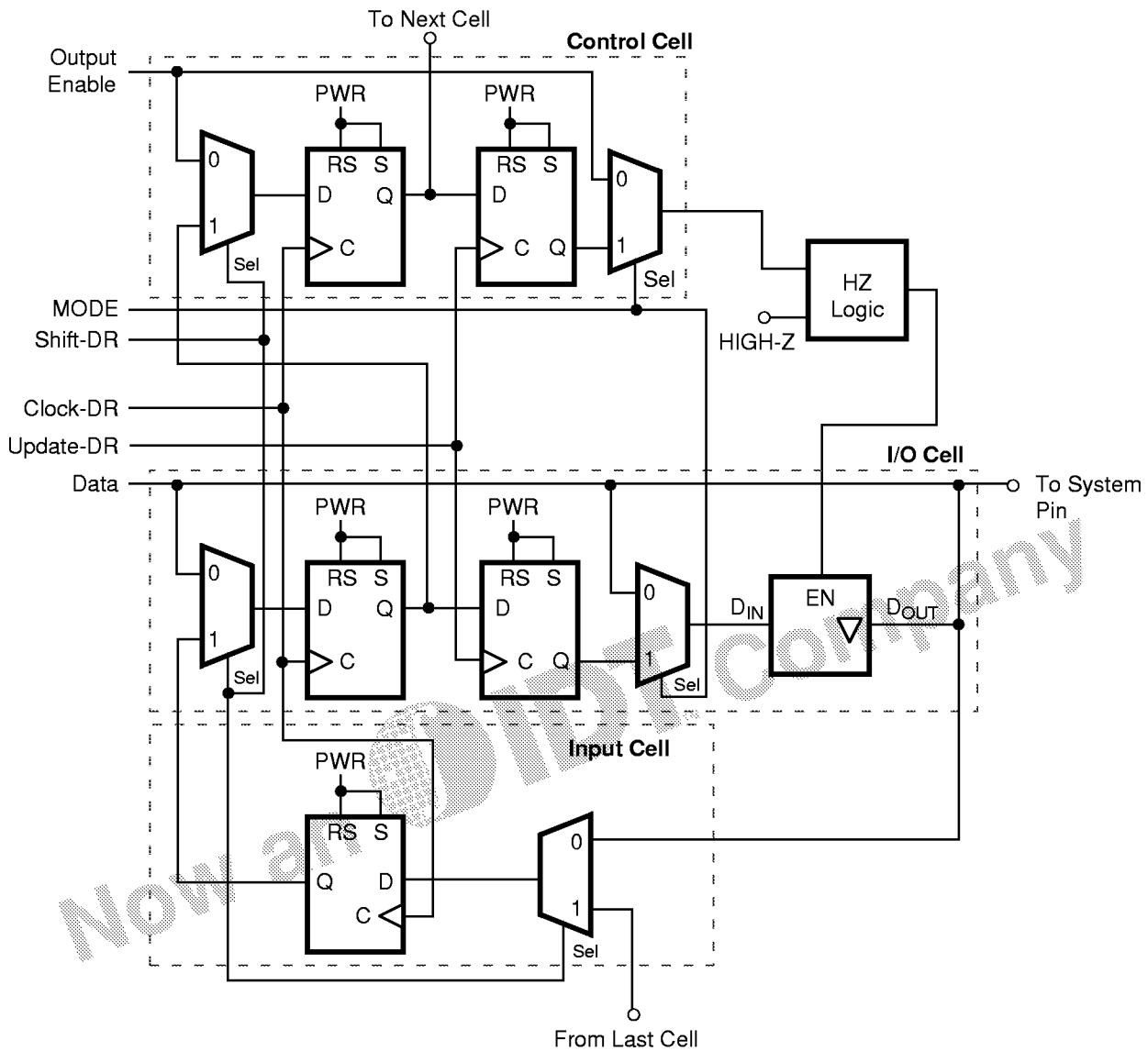
Figure 2. Scan Cell
