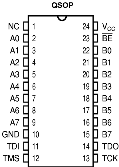
Figure 7. Pin Configuration (All Pins Top View)
