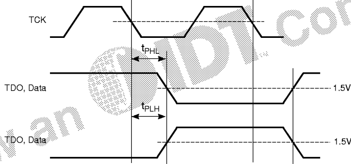
Figure 12. Propagation Delay in Scan Test Operation
