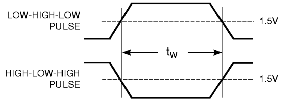
Figure 10. Pulse Width
