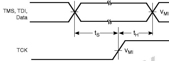
Figure 11. Setup Time, Hold Time
