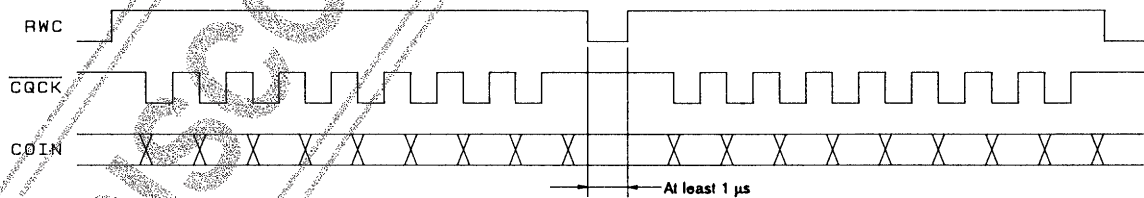
Two-byte commands (RWC set twice) For track checking
