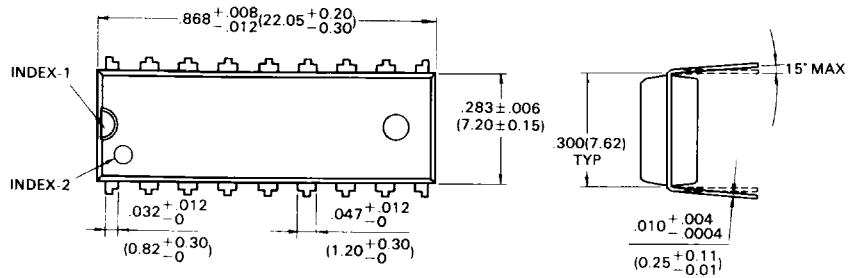
18-LEAD PLASTIC DUAL IN-LINE PACKAGE (CASE No.: DIP-18P-M04)
