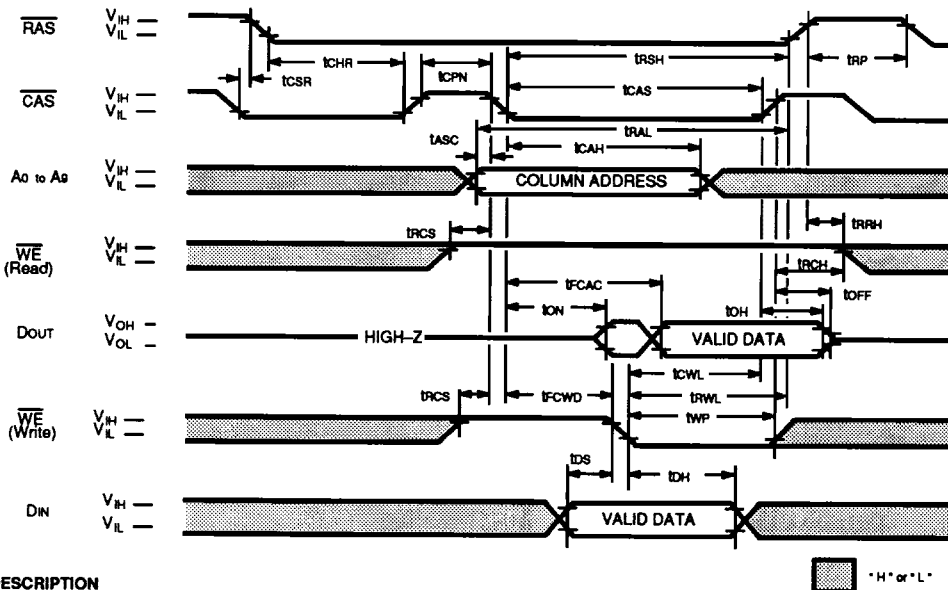
Fig. 13 - \overline{\text{CAS}} -BEFORE- \overline{\text{RAS}} REFRESH COUNTER TEST CYCLE
