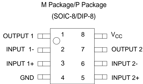
Figure 2. Pin Configuration of AZ358/358C (Top View)
