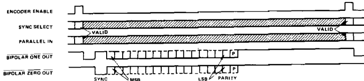
Typical Timing Diagram for a Manchester Encoded UART
