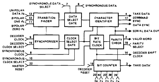
DECODER
