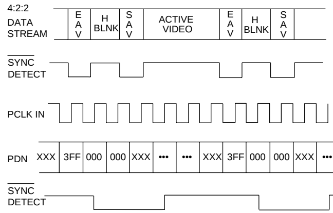
Fig. 5 Timing Diagram
