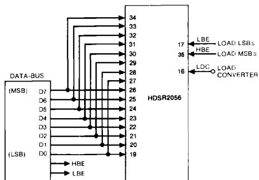
FIGURE 9 Digital Connections for Two-Byte Loading
