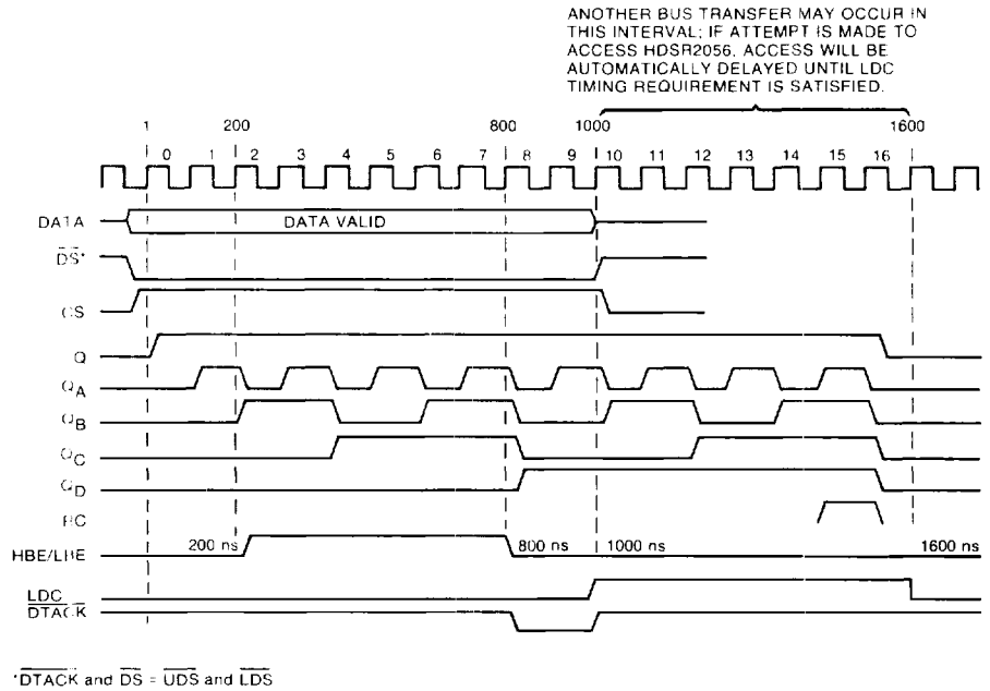
FIGURE 14 16-Bit Microprocessor Interface Timing
