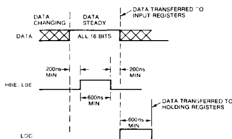
FIGURE 12 Single-Byte Loading
