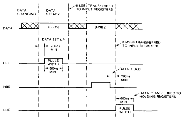
FIGURE 10 Two-Byte Loading
