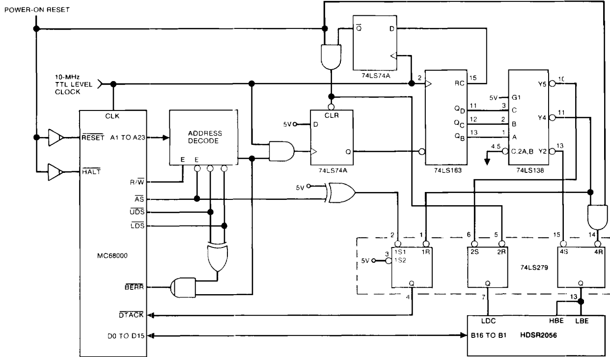
FIGURE 13 Interfacing Digital-To-Synchro/Resolver Converter With 16-Bit Microprocessor.
