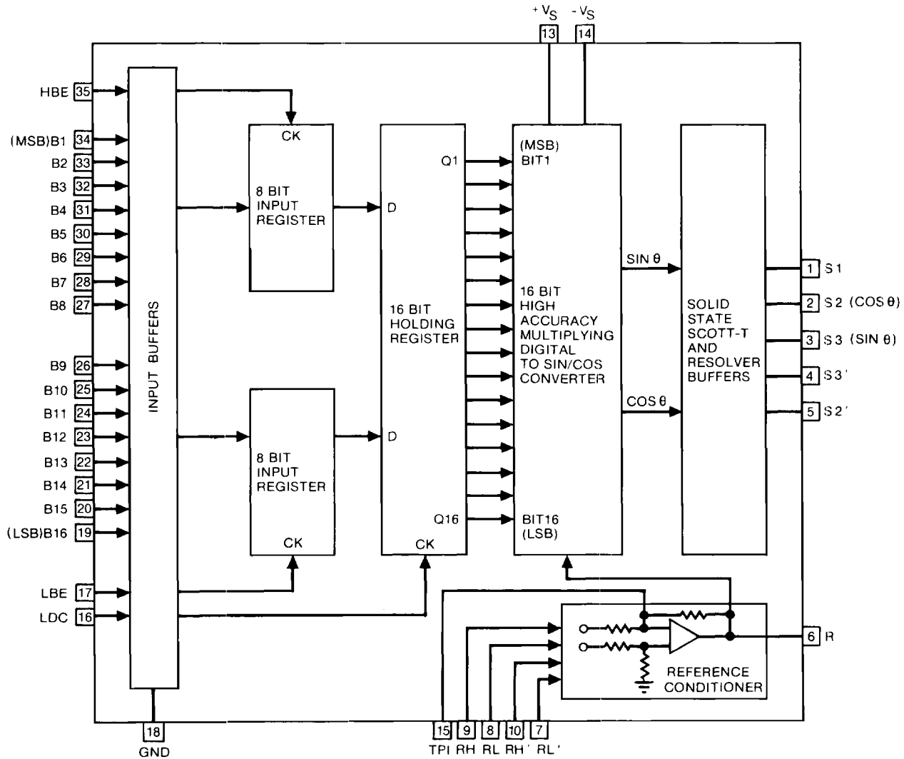
FIGURE 1 2056 Block Diagram
