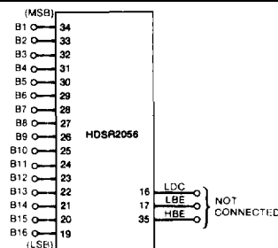
FIGURE 8 Digital Connection for Continuous Operation
