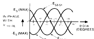
Synchro Output
