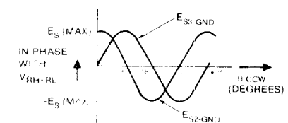
Resolver Output
