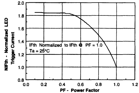
Figure 8. Normalized LED trigger current versus power factor
