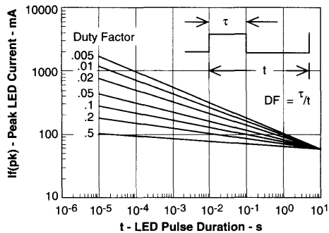
Figure 3. Peak LED current vs. duty factor, Tau
