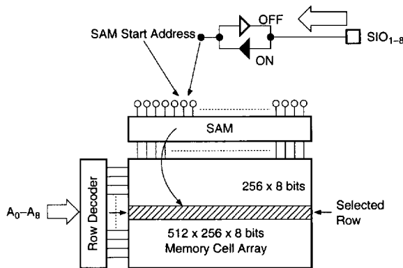
Figure 9. Block Diagram for Write Transfer Operation
