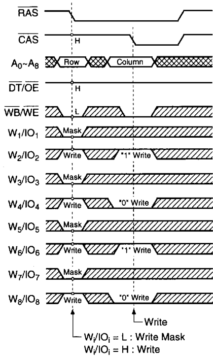
Figure 2. Write-per-bit timing cycle
