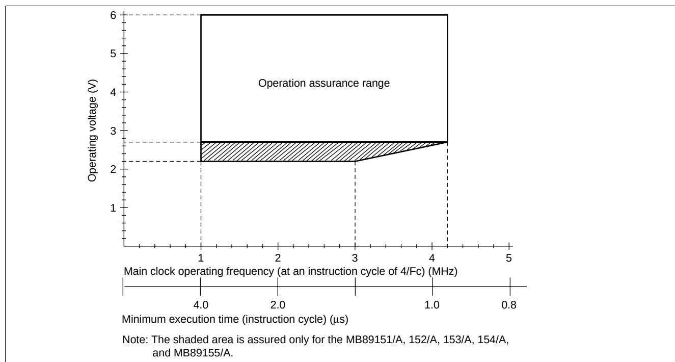
Figure 1 Operating Voltage vs. Main Clock Operating Frequency (MB89P155/PV150, and single-clock MB89151/A, 152/A, 153/A, 154/A, and MB89155/A)
