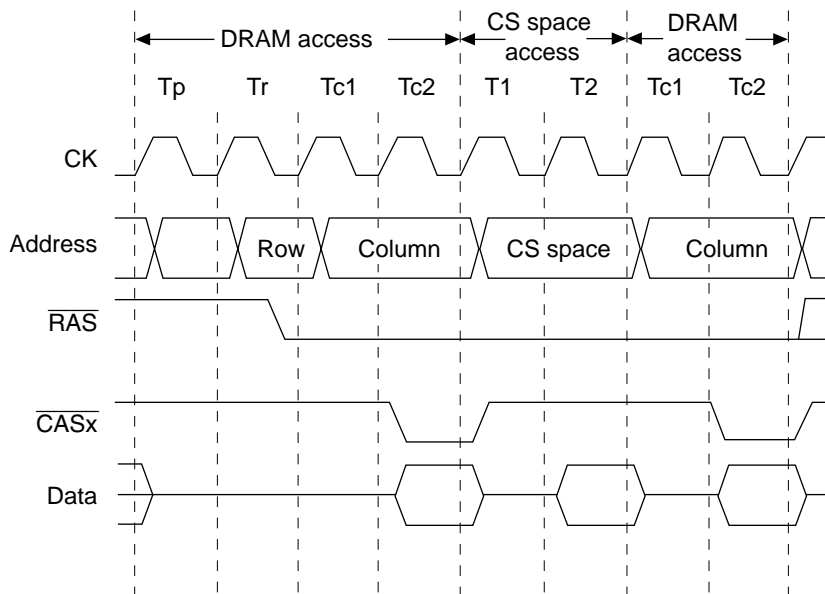
Figure 8.14 RAS Down Mode
