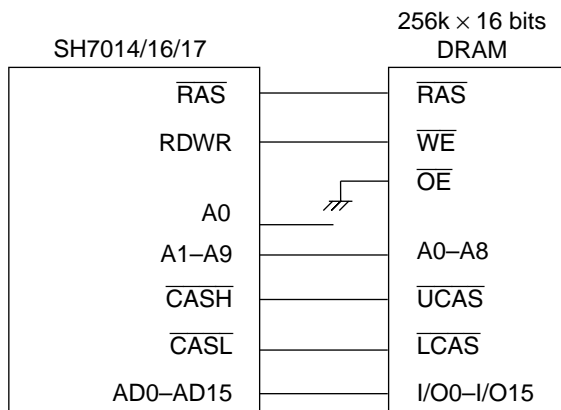
Figure 8.27 16-Bit Data Bus Width DRAM Connection
