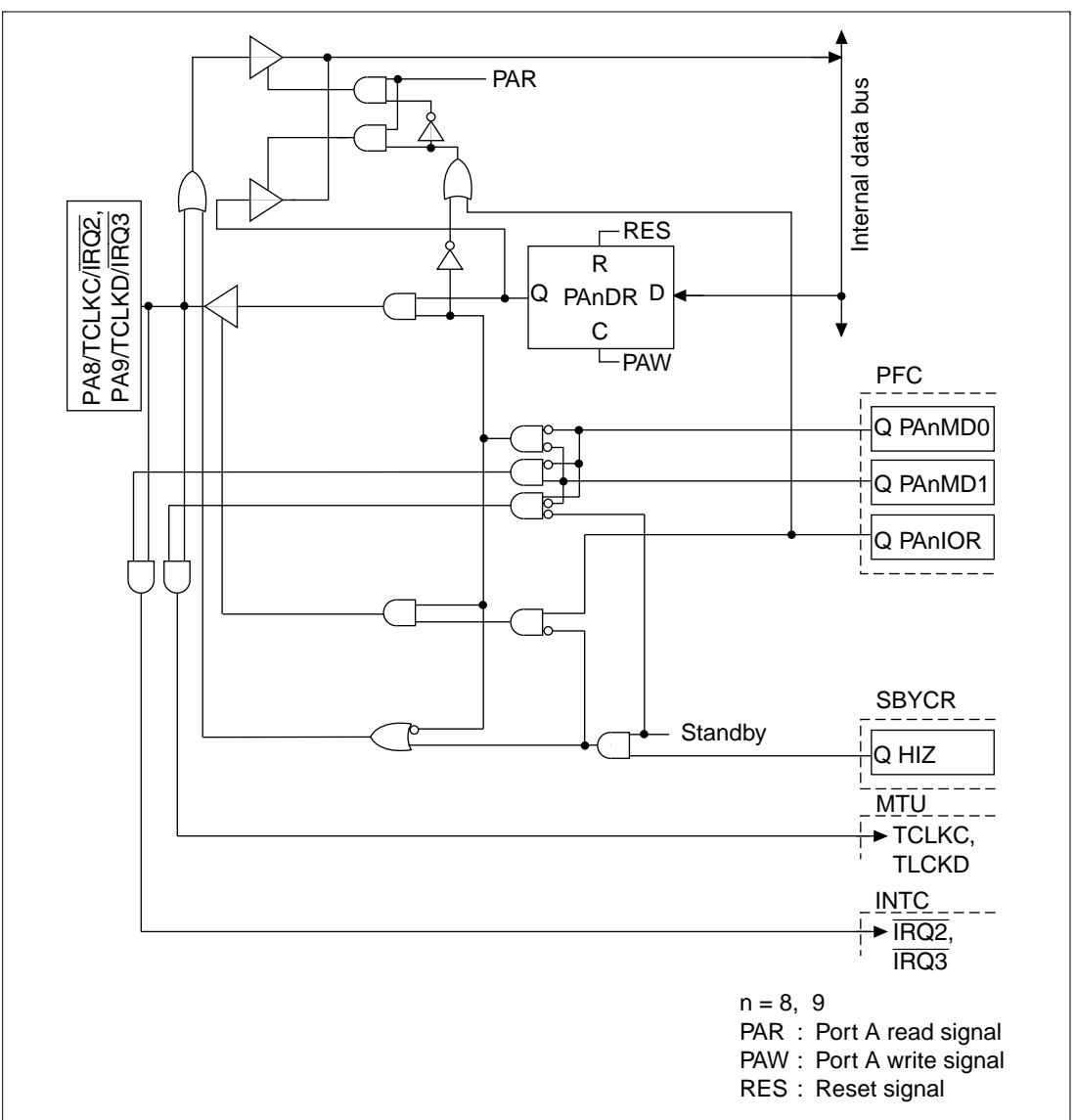
Figure B.5 PAn/TCLKm/IRQx Block Diagram (ZTAT, Mask)
