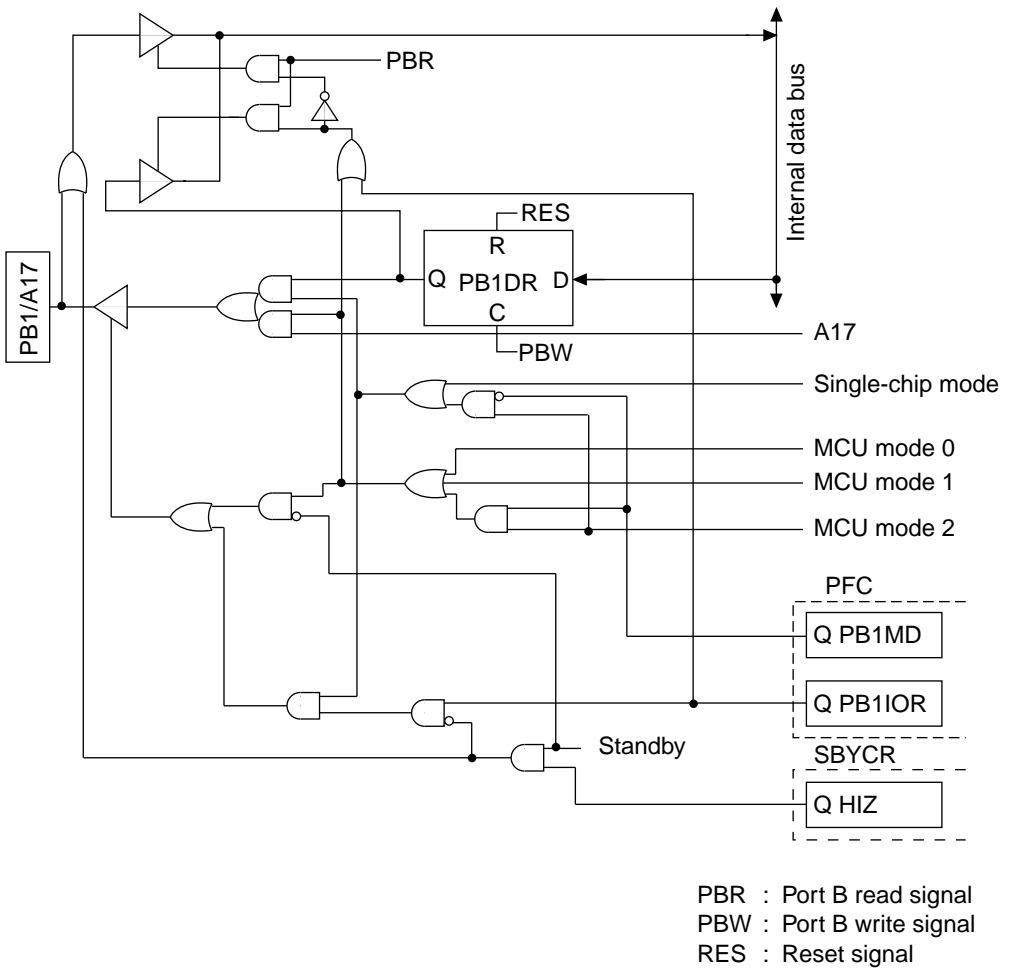
Figure B.11 PB1/A17 Block Diagram (SH7016, SH7017)
