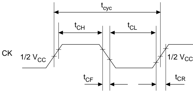
Figure 22.1 System Clock Timing
