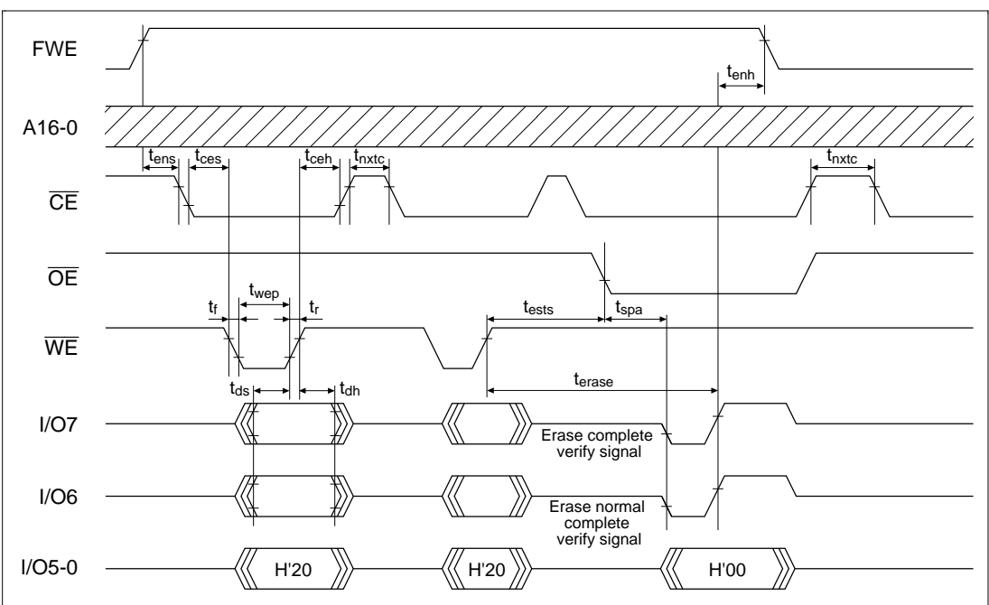
Figure 18.25 Auto-Erase Mode Timing Waveforms
