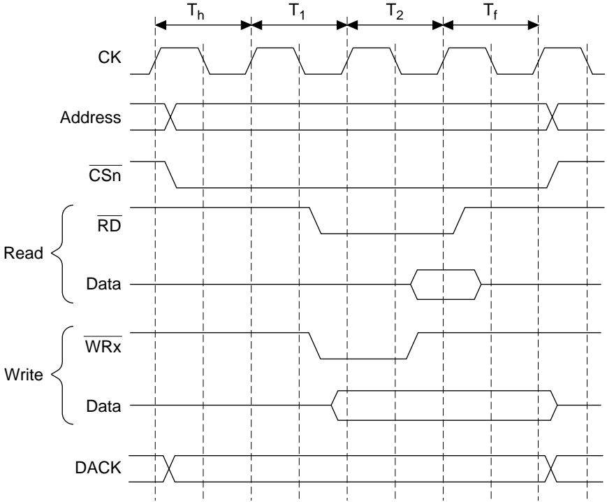
Figure 8.6 \overline{\text{CS}} Assert Period Extension Function
