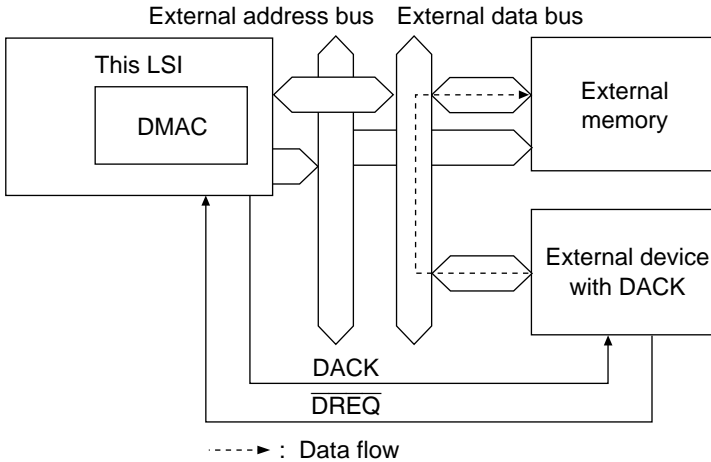
Figure 9.3 Data Flow in Single Address Mode
