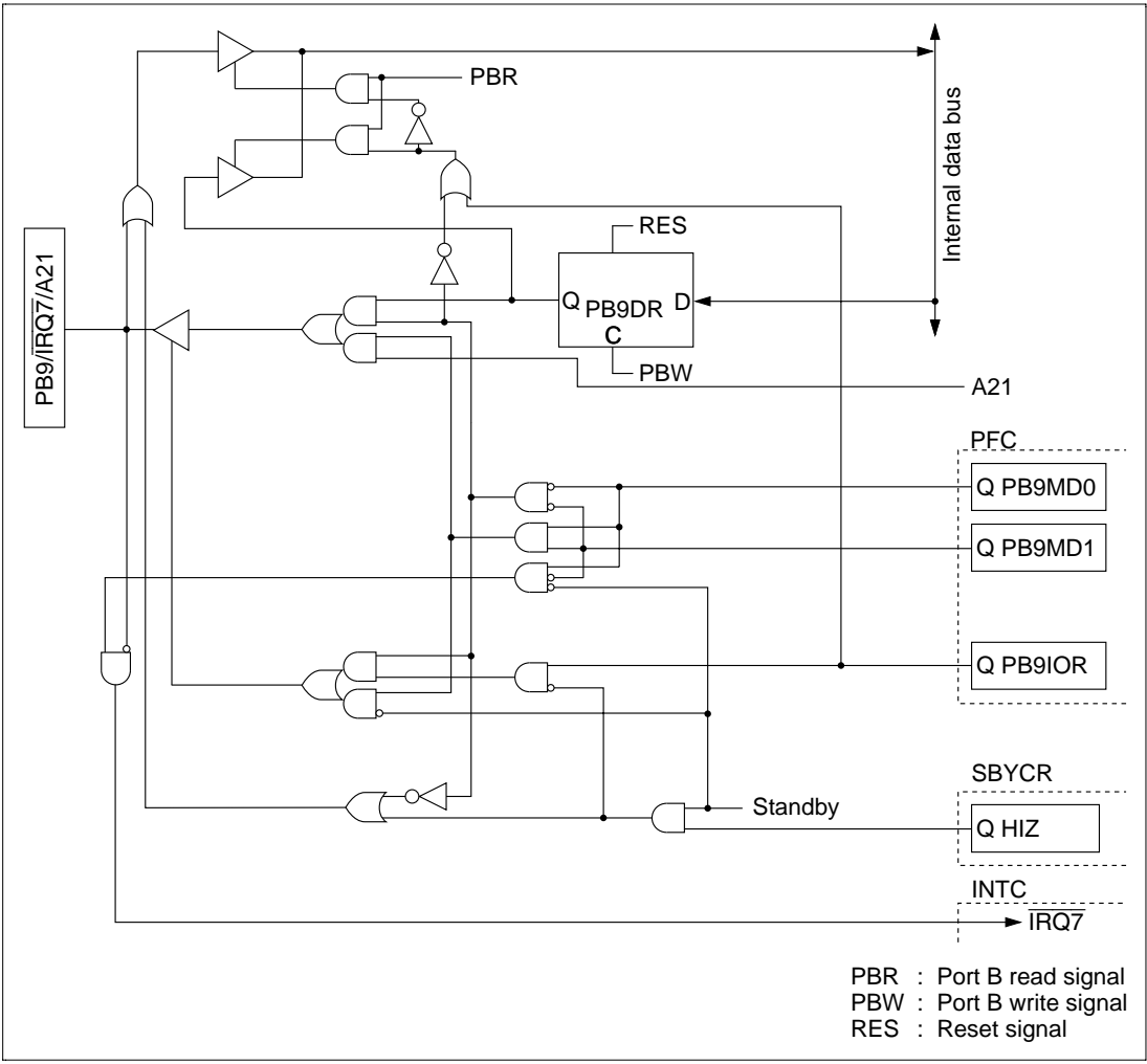
Figure B.15 PB9/ \overline{\text{IRQ7}} /A21 Block Diagram
