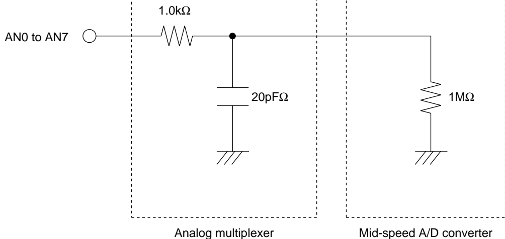
Figure 14.9 Equivalent Circuit for the Analog Input Pins
