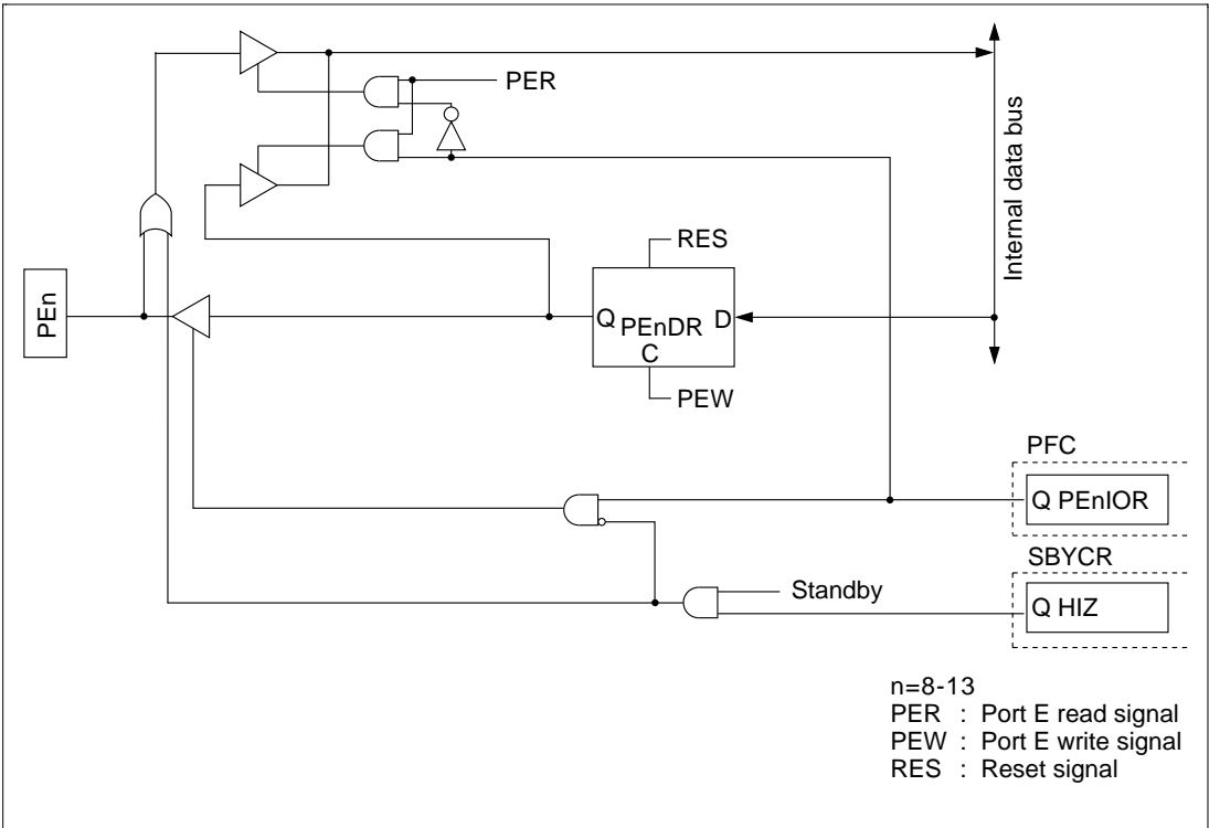
Figure B.19 PEn Block Diagram
