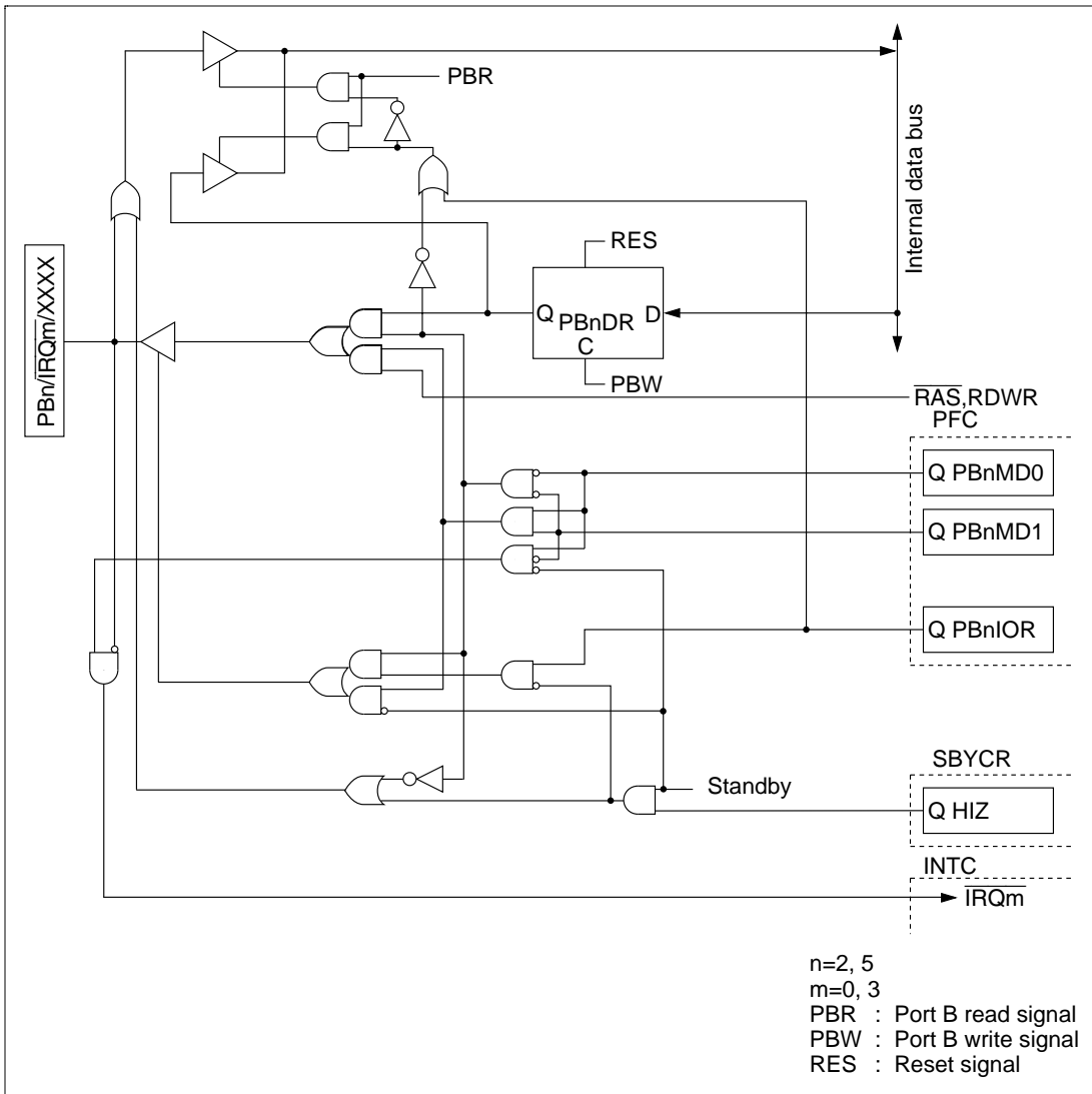
Figure B.16 PBn/IRQm/XXXX Block Diagram
