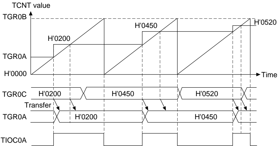
Figure 10.19 Buffer Operation Example (Output Compare Register)
