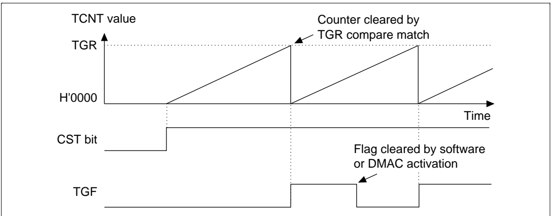
Figure 10.8 Periodic Counter Operation
