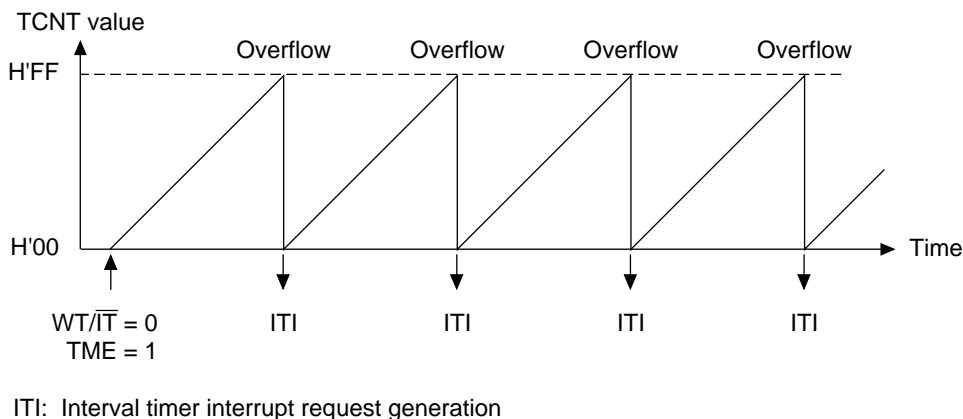
Figure 11.5 Operation in the Interval Timer Mode
