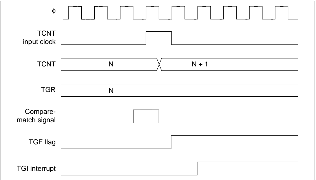
Figure 10.43 TGI Interrupt Timing (Compare Match)
