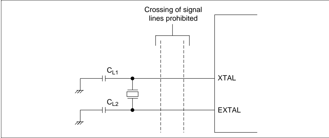
Figure 4.4 Cautions for Oscillator Circuit System Board Design
