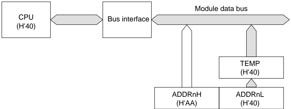
Figure 14.2 ADDR Access Operation (During Reading of (H'AA40))
