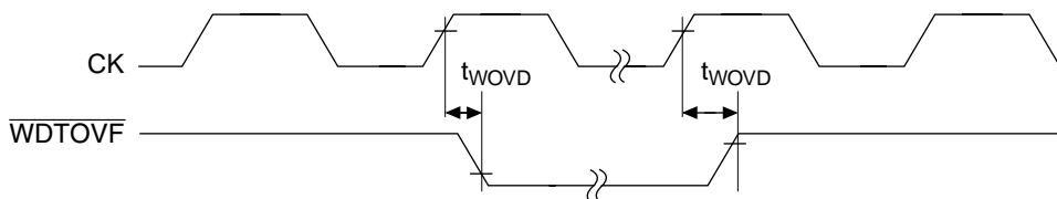
Figure 22.24 Watchdog Timer Timing
