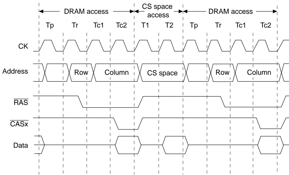
Figure 8.13 DRAM Access Normal Operation (RAS Up Mode)
