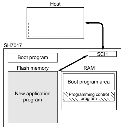
Figure 18.3 Boot Mode
