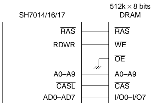
Figure 8.26 8-Bit Data Bus Width DRAM Connection
