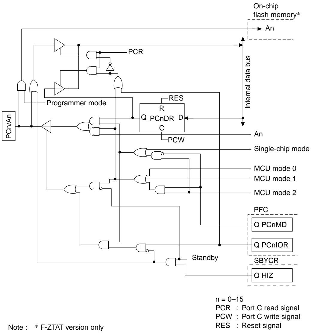
Figure B.17 PCn/An Block Diagram
