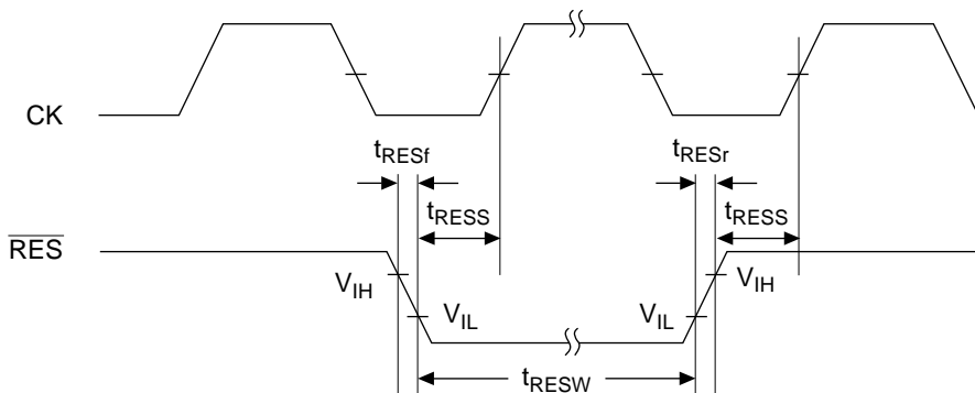
Figure 22.4 Reset Input Timing
