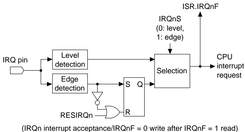
Figure 6.2 External Interrupt Process
