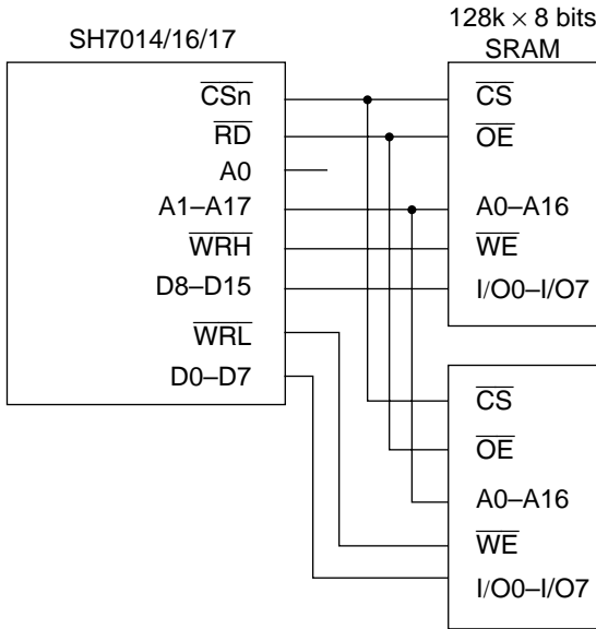
Figure 8.25 16-Bit Data Bus Width SRAM Connection
