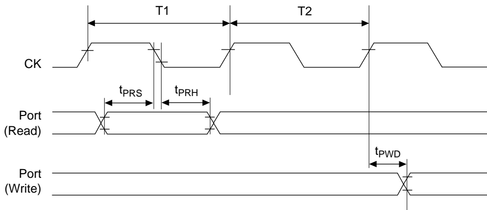
Figure 22.23 I/O Port I/O Timing
