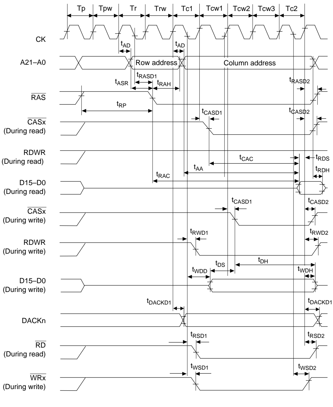
Figure 22.12 DRAM Cycle (Normal Mode, 3 Waits, TPC = 1, RCD = 1)
