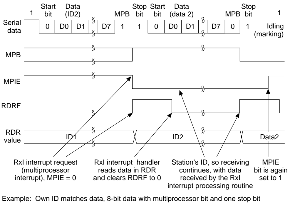
Figure 12.16 Example of SCI Receive Operation (ID Matches)
