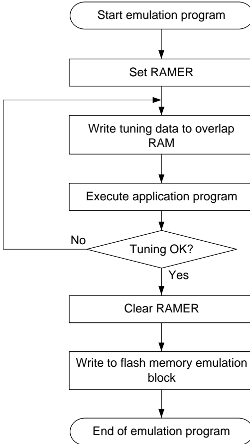
Figure 18.16 Flowchart for Flash Memory Emulation in RAM
