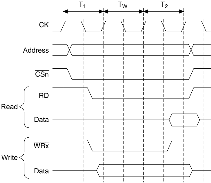
Figure 8.4 Wait Timing of Ordinary Space Access (Software Wait Only)
