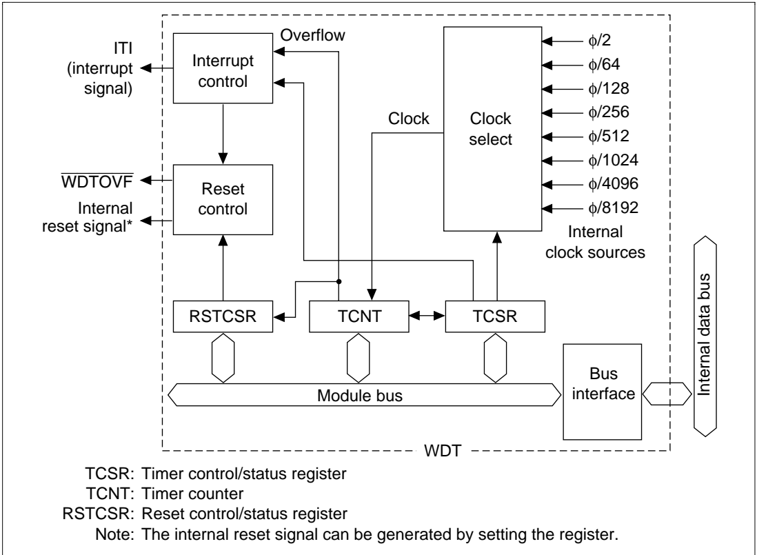
Figure 11.1 WDT Block Diagram
