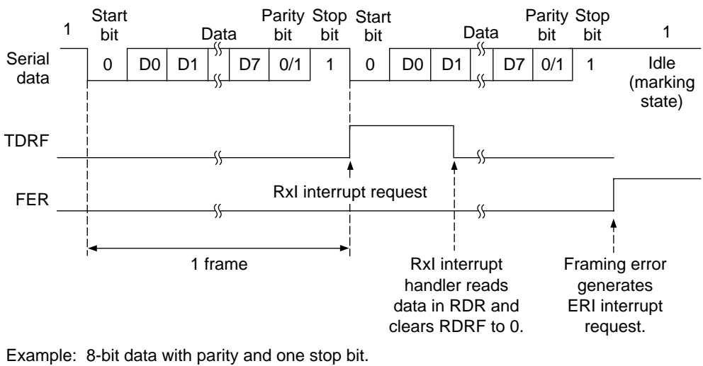
Figure 12.9 SCI Receive Operation
