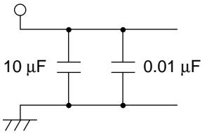
Figure 14.8 Example of Analog Input Pin Protection Circuit
