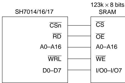
Figure 8.24 8-Bit Data Bus Width SRAM Connection
