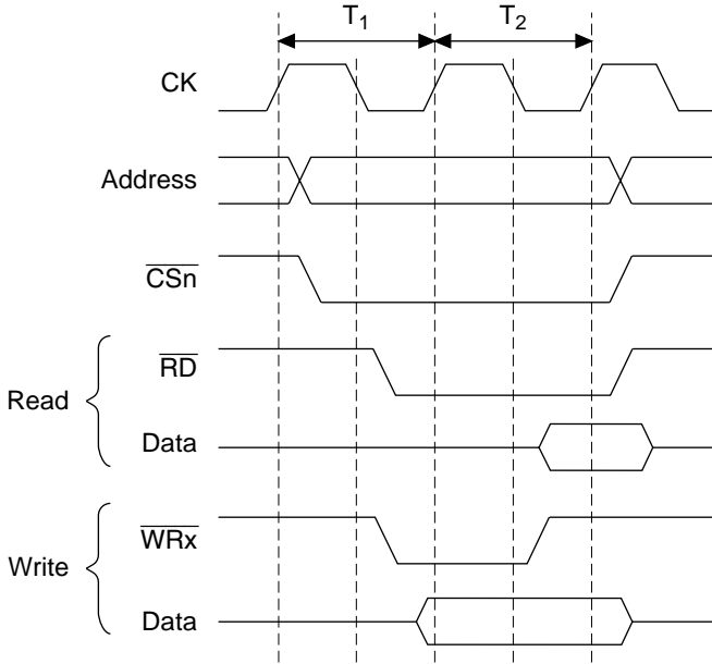
Figure 8.3 Basic Timing of Ordinary Space Access
