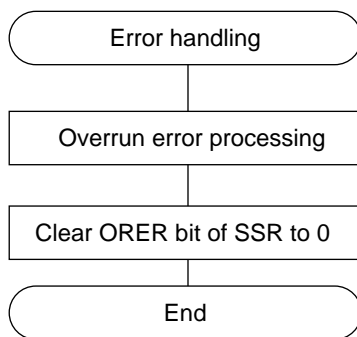
Figure 12.22 Sample Flowchart for Serial Receiving (2)
