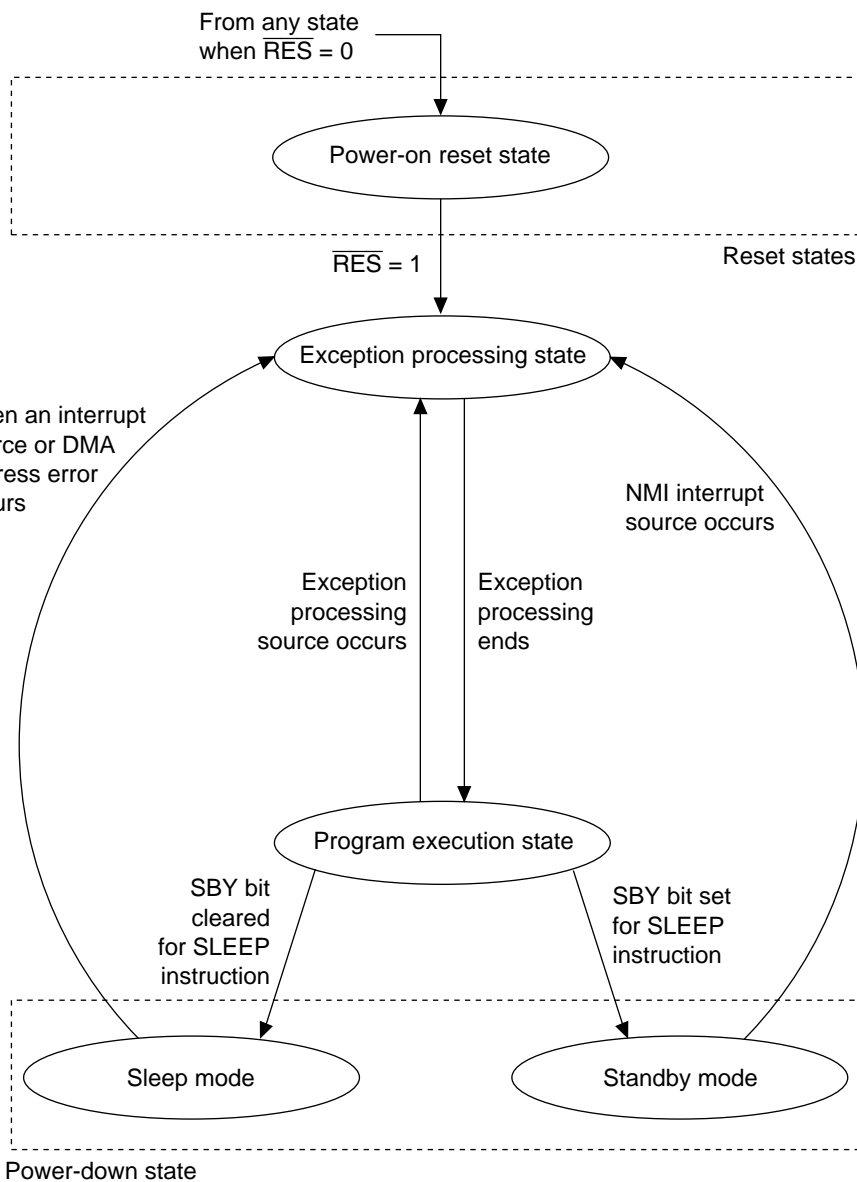
Figure 2.6 Transitions between Processing States
