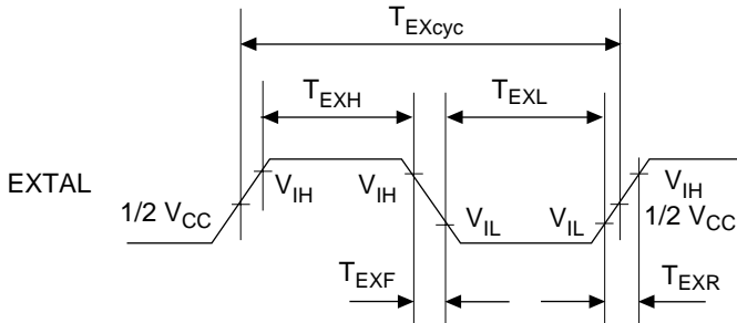
Figure 22.2 EXTAL Clock Input Timing
