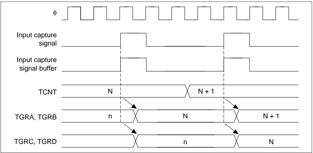
Figure 10.42 Buffer Operation Timing (Input Capture)
