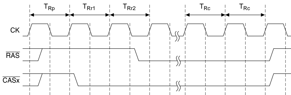
Figure 8.16 Self-Refresh Timing
