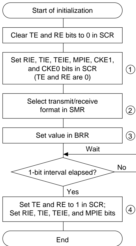
Figure 12.18 Sample Flowchart for SCI Initialization
