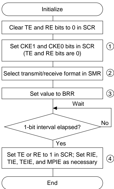
Figure 12.4 Sample Flowchart for SCI Initialization
